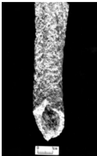
Grade 5: Heavy erosion (in this case by root action) across whole surface, completely masking normal surface morphology, with some modification of profile.
