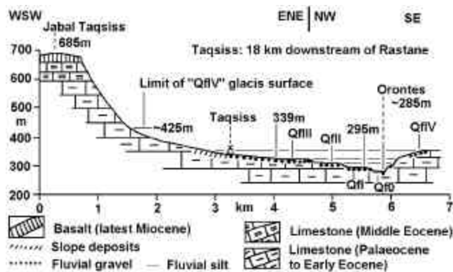
Figure 7. Profile at Taqsiss, indicating ~400 m of incision since the eruption of basalt, probably in the latest Miocene, adapted from part of Figure 9 of Besançon and Sanlaville 3 . Jabal Taqsiss is located just north of the NE corner of Figure 1.
