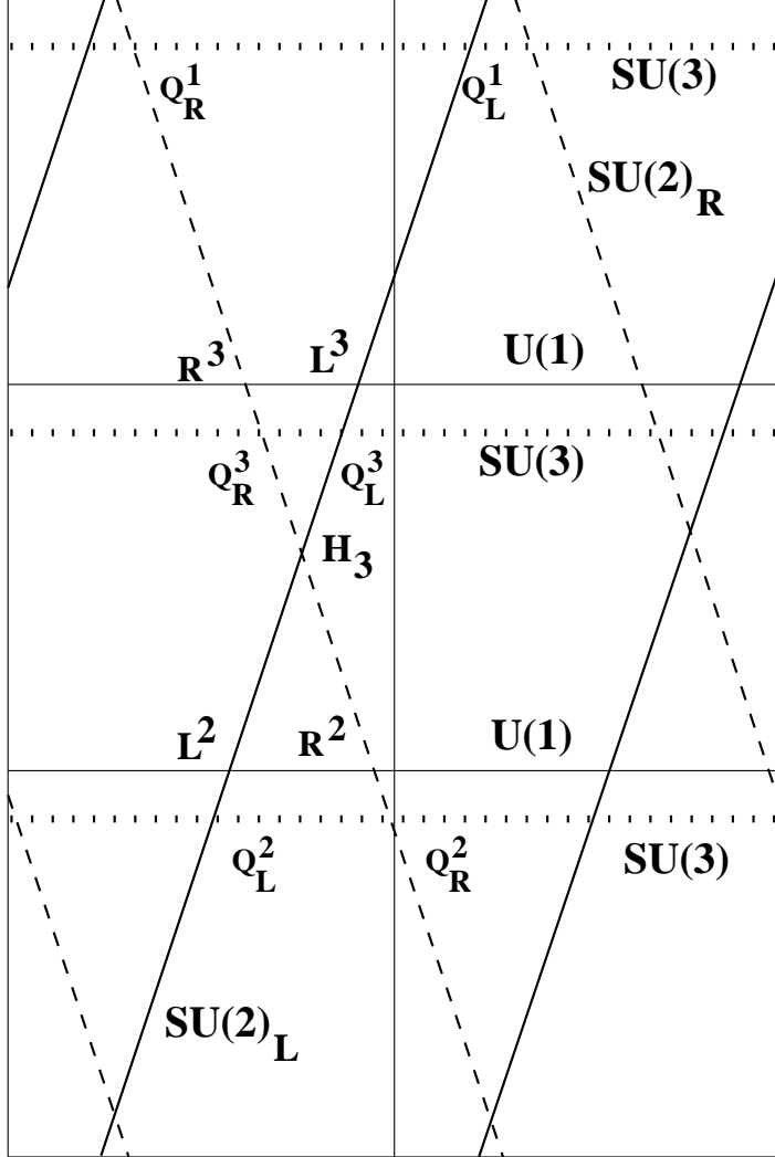
Figure 4: The SU(3) \times SU(2)_L \times SU(2)_R \times U(1) model of Fig. 2. Several torus fundamental domains are shown to highlight the relative size of the different Yukawa couplings. To avoid clutter, we do not show all the copies of the branes. Also, we only highlight the Yukawa couplings involving the Higgs field H_3 , hence do not show other fields living at the relevant intersections. World-sheets giving rise to quark (lepton) Yukawa couplings correspond to triangles with one vertex ( H_3 ) containing the Higgs and other two vertices Q_L^i, Q_R^i ( L^i, R^i ) containing the quarks (leptons).
