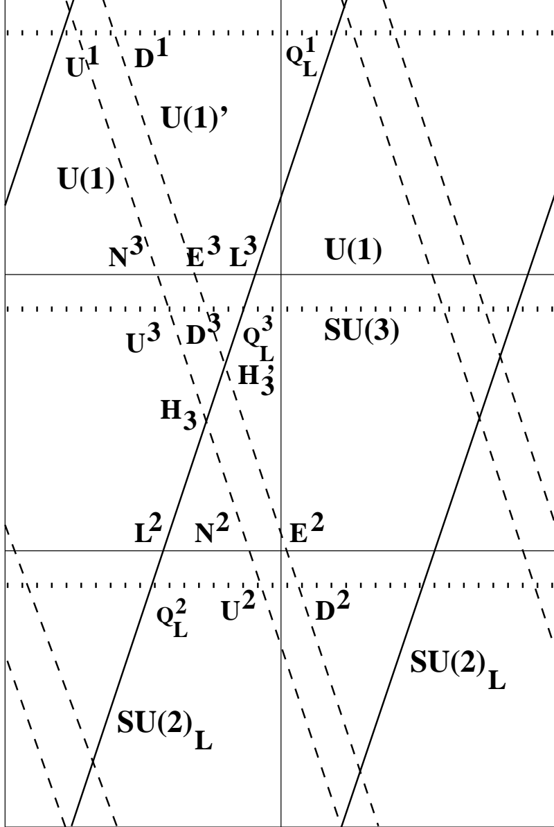
Figure 5: A standard model-like configuration obtained from that in Fig. 4 by splitting the SU(2)_R D4-branes into two parallel U(1) -branes. Now the size of the triangles corresponding to u- and d-quark Yukawa couplings are different.
