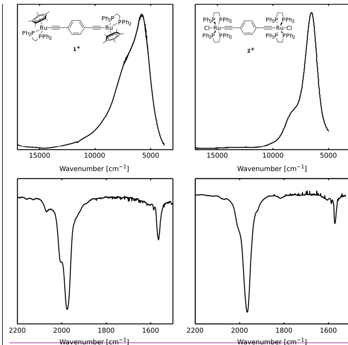
Figure 3. The spectroelectrochemically generated NIR (upper) and IR (lower) spectra of [1]^+ (left) [24] and [2]^+ (right) in DCM / 0.1 M \text{NBu}_4\text{BF}_4 .
