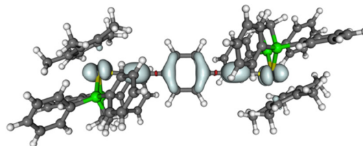
Figure 4. Spin-density isosurface plot ( \pm 0.002 a.u.) of trans - [1]^+ .
