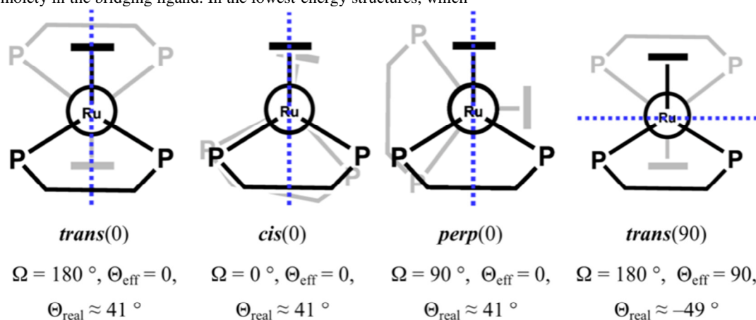
Figure 2. Schematic relative orientation of the metal redox centers (black and grey) and the bridge phenyl plane (dashed blue) of [1-Me] + at various values of \Omega , \Theta_{\text{eff}} and \Theta_{\text{real}} (similar values hold for [2-Me] + ).
