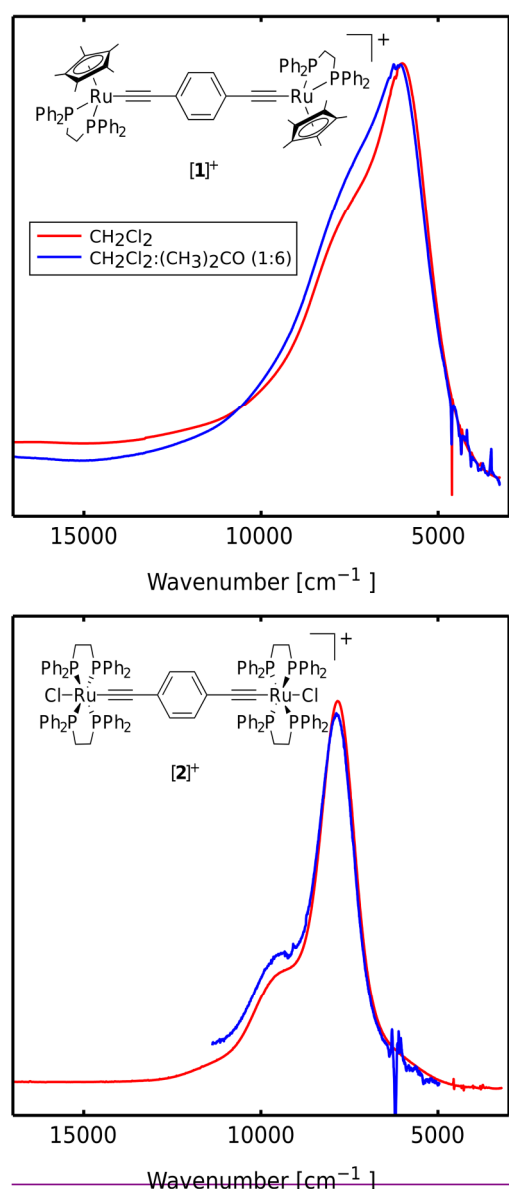
Figure 11. Overlay plots of the NIR spectra of [\mathbf{1}]^+ and [\mathbf{2}]^+ obtained by chemical oxidation in differing solvent mixtures.
