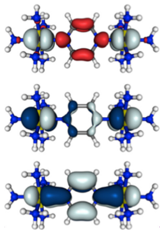
Figure 14. Isosurface plots of the spin-density (top, \pm 0.002 a.u.) and \beta -SOMO (middle)/ \beta -HOMO (bottom) ( \pm 0.03 a.u.) of [3]^{5+} (BLYP35/def2-SVP/COSMO(MeCN) level).
