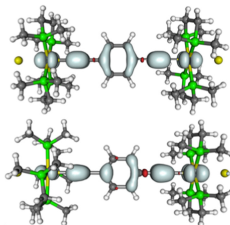
Figure 12. Spin-density isosurface plots ( \pm 0.002 a.u.) of deloc - [\mathbf{2-Me}]^+ (top) and sb - [\mathbf{2-Me}]^+ (bottom) (BLYP35/def2-SVP/COSMO(DCM) level).
