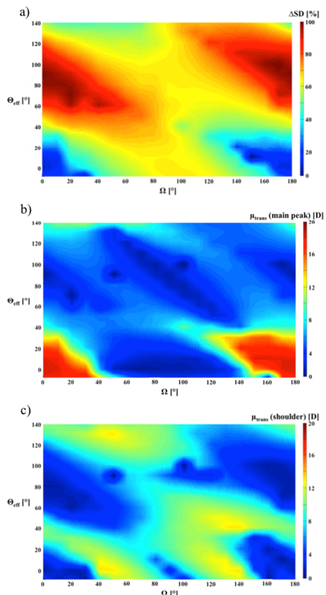
Figure 9. Properties (BLYP35/def2-SVP/COSMO(DCM) level) as function of conformational phase space of [\mathbf{1-Me}]^+ . a) Color plot of Mulliken spin-density differences, \Delta\text{SD} , between the two \text{Cp}^*(\text{dmpe})\text{Ru-C}\equiv\text{C} units. 0 % indicates fully delocalized and 100 % fully localized distributions (top). b) TDDFT transition dipole moment \mu_{\text{trans}} of the main \pi\rightarrow\pi^* excitation at around 6000\text{ cm}^{-1} (middle). c) TDDFT transition dipole moment of the IVCT excitation at higher energies 7350\text{-}9450\text{ cm}^{-1} (bottom). For \Omega = 50^\circ , \Theta_{\text{eff}} = 91.7^\circ and for \Omega = 100^\circ , \Theta_{\text{eff}} = 101.6^\circ , TDDFT did not converge, and the values were set to 0 (“holes”).
