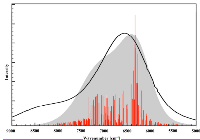
Figure 13. Computed Boltzmann-weighted TDDFT stick spectra (red) with Gaussian broadened envelope ( \sigma = 300 cm -1 , FWHM = 706.4 cm -1 , grey) for [2-Me] + compared to experimental IVCT band [23] (black line) of [2] + .
