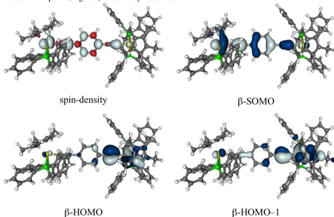
Figure 10. Isosurface plots of the spin-density (top left, \pm 0.002 a.u.) and key orbitals ( \pm 0.03 a.u.) involved in the NIR excitations of conformer perp -[1-Me] + (BLYP35/def2-SVP/COSMO(DCM)).
