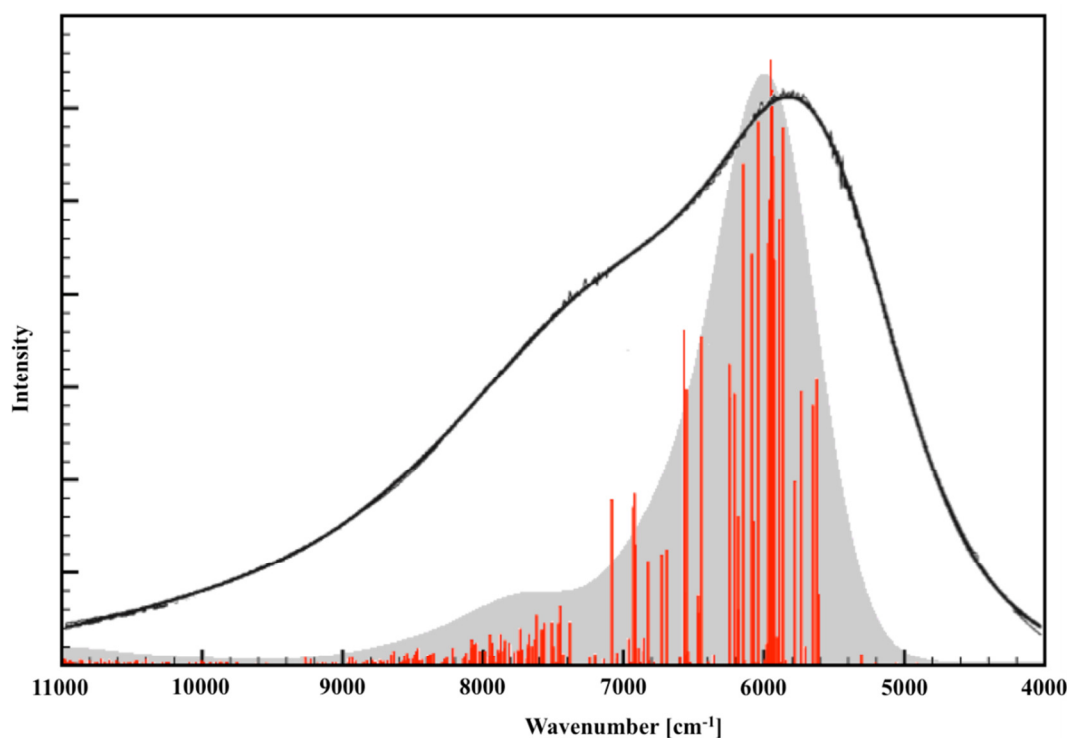
Figure 8. Computed Boltzmann-weighted TDDFT stick spectra (red)—with Gaussian broadened envelope ( \sigma = 300\text{ cm}^{-1} , FWHM = 706.4\text{ cm}^{-1} , grey) for [1\text{-Me}]^+ compared to experimental IVCT band [24] (black line) of [1]^+ .
