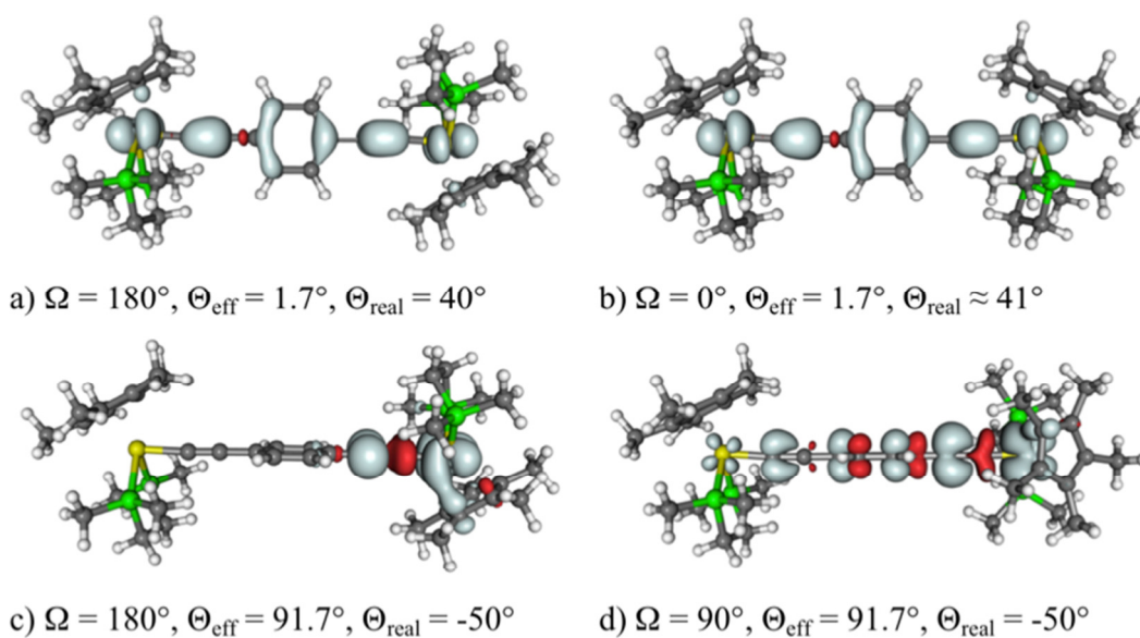
Figure 7. Spin-density isosurface plots ( \pm 0.002 a.u.) of [1\text{-Me}]^+ for different points on the PES (BLYP35/def2-SVP/COSMO(DCM) level; cf. Figure 3 for the definition of dihedral angles and Figure 6 for the PES).
