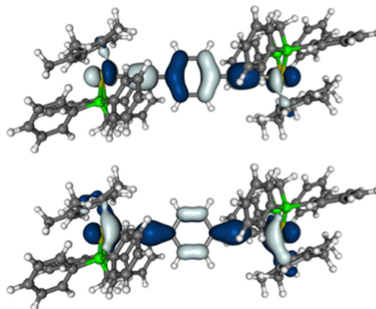
Figure 5. Isosurface plots ( \pm 0.03 a.u.) of the \beta -SOMO (top) and \beta -HOMO (bottom) of trans -[1] + .
