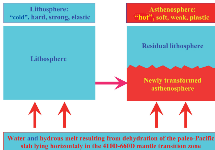
Fig. 12. Illustration of the concept of basal hydration-weakening as an effective mechanism to have caused the lithosphere thinning beneath eastern China (Niu 2005b, 2006). The basic physical difference between the lithosphere and asthenosphere lies in the physical properties as indicated. Water and hydrous melt derived from dehydration of the paleo-Pacific slab in the transition zone (Fig. 10) will convert the basal portion of the lithosphere into asthenosphere, accomplishing the lithosphere thinning.
