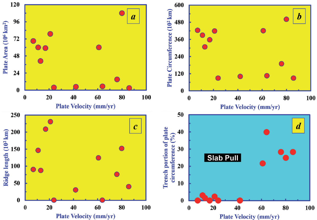
Fig. 2. In search of the driving force for plate motion, Forsyth and Uyeda (1975) recognized that the velocity of plate motion is independent of plate size (a), circumference (b) and ridge length (c), but is related to the trench portion of a plate circumference (d), suggesting that Slab Pull due to gravity is the primary force for plate motion. From left to right, the 12 data points are rigid plates of Eurasia (EU), North America (NA), South America (SA), Antarctica (AN), Africa (AF), Caribbean (CA), Arabia (AR), India-Australia (IA), Philippines (PH), Nazca (NZ), Pacific (PA) and Cocos (CO) as shown in Fig. 1.
