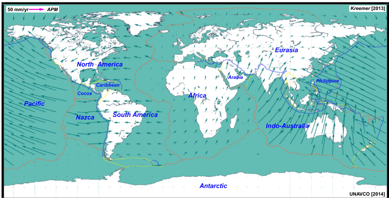
Fig. 1. World map contrasting oceans (ocean blue) and continents (white), also showing (1) the 12 “rigid” plates of varying size and nature as labeled (oceanic plates, continental plates and ocean+continent plates) (e.g., Forsyth & Uyeda 1975); (2) plate boundaries: divergent (brown; ocean ridges, back-arc spreading centers), convergent (blue; subduction zones indicated by trenches and continental collision zones), large transforms (yellow); and (3) the present-day plate motion vectors using the “sub-asthenosphere” reference frame (APM; from UNAVCO: http://jules.unavco.org/Voyager/GEM_GSRM ). Note that both relative and “absolute” plate motion vectors depend on model references chosen. Also note (1) that the northern and western Pacific has well-developed back-arc basins, yet the eastern Pacific is characterized by active continental margins with oceanic lithosphere subducting beneath continents (except for the segment separated by the San Andreas transform in north America) without back-arc basins; and (2) that the Indo-Australian is a single giant ocean-continent plate in terms of the rigid plate concept.
