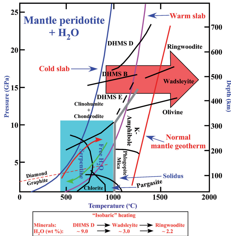
Fig. 14. Phase diagram of mantle peridotite to show mineral phases and their stability in the subducting/subducted oceanic lithospheric mantle under upper mantle conditions (after Williams & Hemley 2001). Prior to subduction, the oceanic lithospheric mantle has experienced considerable serpentinization, including near-ridge shallow (< 20km) hydrothermal metamorphism (Dick 1989; Niu & Hekinian 1997; Niu 1997, 2004) and serpentinization at depths (~50 km) caused by seawater penetration through extensional faults at trench outer-rise (Ranero et al. 2003; Dobson et al. 2002; Kerrick 2002), and thus contain abundant water (up to 13wt% in serpentine phases). Considering the thermal structure of the subducting slab, subduction-dehydration is necessarily incomplete (Niu 2004, 2005b). Antigorite serpentine is experimentally shown to be stable under P \leq 7.5 GPa and T \leq 800^\circ\text{C} (Ulmer & Trommsdorff 1995) in the subducting slab, and can transform under higher pressures into dense hydrous magnesium silicate phases (DHMS: A, B, D-F-G and G) stable over a greater pressure range (~5 to 50 GPa; Frost 1999; Williams & Hemley 2001) with abundant water (~3 to 20 wt.%) that can be transported to the deep mantle (Kuroda & Irifune 1998). As indicated by the thick pink arrow and explanation in the bottom panel, the transition zone slab will undergo isobaric heating with time and release water (most likely in the form of hydrous melt) by changing into progressively water-poor mineral phases. The water (hydrous melt) so released will rise and percolate through the upper mantle to facilitate the formation and maintenance of the LVZ (see Fig. 15 below), which is in fact the process of lithosphere thinning and related magmatism.
