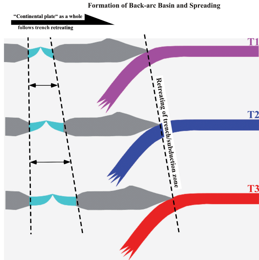
Fig. 9. Cartoon illustrating back-arc basin formation and growth. The drifting overriding continental plate that is under extension (Fig. 8) can develop within its interiors extensional basins on land and even back-arc basins with spreading centers. It is thus conceptually clear that the “Island Arc System” is simply split from the margin of the overriding continental plate. That is, the “Island arc system” must have its basement of continental origin. Also note that back-arc spreading centers can evolve to large open ocean basins and the “Island arc systems” can become micro continents.
