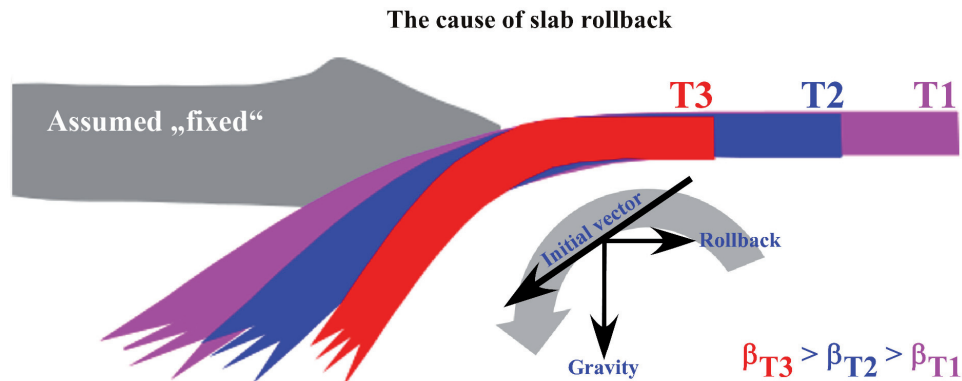
Fig. 7. Cartoon illustrating the cause of slab rollback. Figures 4e and 5a show that F_B is the principal force for subduction initiation and is inversely related to the dip angle (i.e., F_B \propto -\beta ). That is, a smaller dip angle \beta (thus a larger triangular volume beneath the fault plane in Fig. 4d, and a greater F_B ) favors subduction initiation. However, once subduction began, the slab tends to rotate vertically under gravity ( \beta_{T3} > \beta_{T2} > \beta_{T1} ). This is the concept of slab rollback. Note that the trench position is actually not fixed, but retreating under gravity (see Fig. 8).
