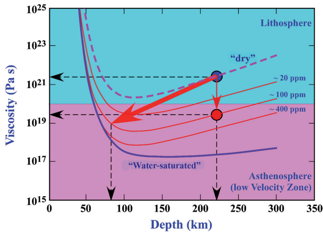
Fig. 13. Experimental data showing the effect of water content on the upper mantle peridotite viscosity (after Karato 2003). The upper light blue portion lies in the “rigid” range of lithospheric viscosity ( > 10^{20} Pa s), and the lower purple portion lies in the “plastic” range of asthenospheric viscosity ( < 10^{20} Pa s). The seismic low velocity zone (LVZ) has the viscosity of \leq 10^{19} Pa s (Hirth & Kohlstedt 1996; Karato 2003). Assuming the North China Craton in eastern China was \sim 220 km thick (e.g., Xu 2001) and relatively dry with a viscosity of \sim 3 \times 10^{21} Pa s (e.g., the blue solid circle) prior to the thinning, addition of small amount of water (e.g., 100 ppm, dissolved in the nominally anhydrous minerals like olivine) will reduce the bulk viscosity of the mantle lithosphere by two orders of magnitude, \sim 3 \times 10^{19} Pa s (red solid circle), giving it the asthenosphere/LVZ property, i.e., the “rigid” basal portion of the mantle lithosphere has been thinned with the upper \sim 80 km left at present. In fact, the paleo-Pacific slab in the mantle transition beneath eastern China can provide more than needed water (Niu 2005b, 2006).
