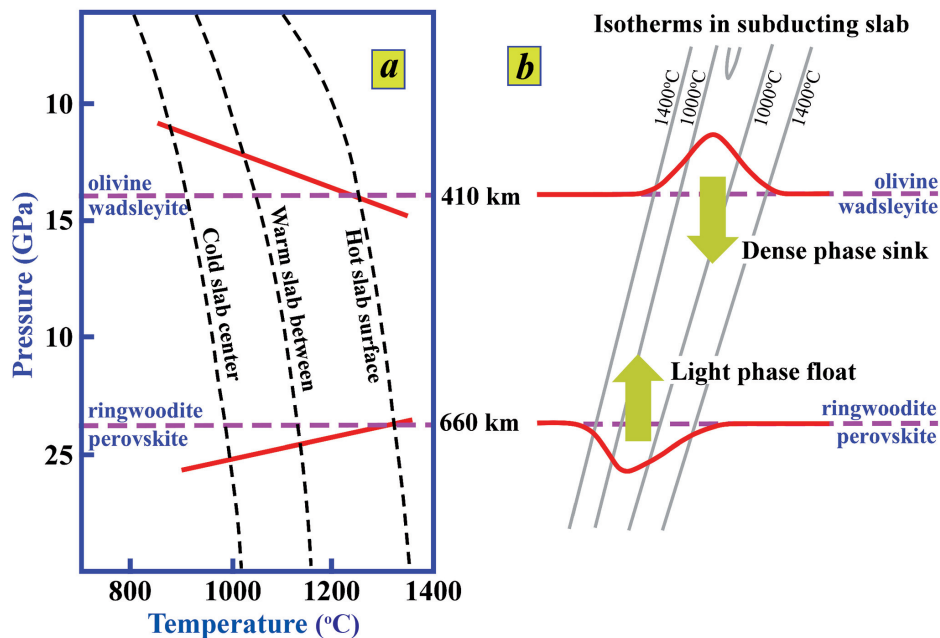
Fig. 3. a. Schematic phase diagram showing the two major phase transitions at depths of 410 km and 660 km, respectively, from low density phase (olivine < 410 km; ringwoodite < 660 km to high density phase (wadsleyite > 410 km; perovskite > 660 km). The positive Clapeyron slope of the 410 km phase transition makes the colder subducting slab change to denser phase at a shallower depth, whereas the negative Clapeyron slope of the 660 km phase transition makes the colder slab change to denser phase at a deeper depth (Ringwood 1991; Irifune & Ringwood 1993; Bina & Helffrich 1994; Agee 1998; Frost 1999). As a result, as shown in b , the density of the subducting slab at 410 km becomes denser than the ambient mantle, facilitating the slab to sink, promotes Slab Pull , and thus enhances the plate driving force. The cold subducting slab at 660 km, however, becomes less dense than the ambient mantle, inhibiting the slab to sink into the lower mantle.
