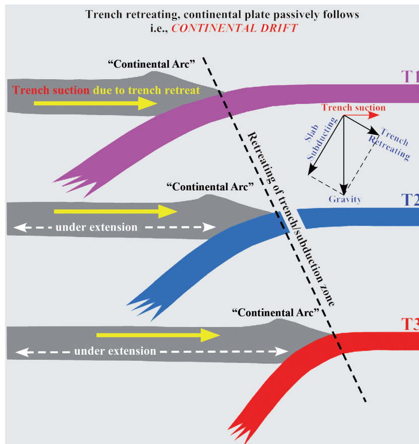
Fig. 8. Cartoon illustrating trench retreat and continental drift. Under gravity, slab will roll back (Fig. 7), and importantly, subduction zone will necessarily move seawards or retreat, which is often described as “trench retreating” because the trenches are surface expressions of subduction zones. The dashed line indicates the newer position of the trench/subduction zone with time: T1 \rightarrow T2 \rightarrow T3 . Importantly, the overriding continental plate will passively follow the retreating trench, which may be termed as the result of trench suction (Forsyth & Uyeda 1975). That is, continental drift is a passive response to subduction. Also note that the drifting overriding continental plate is under extension.
