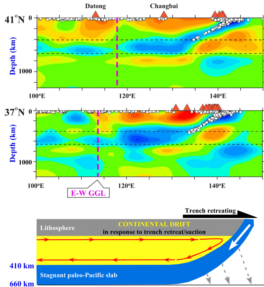
Fig. 10. Top, western Pacific-eastern China mantle seismic tomography across two sections at the latitude of 41°N and 37°N, showing the paleo-Pacific slab lying horizontally in the mantle transition zone between the 410 km and 660 km seismic discontinuities (after Zhao & Ohtani 2009). The pink dashed lines indicate the position of the East-West great gradient line (GGL) as shown in Figure 11, which is also termed North-South gravity lineament (NSGL; Xu 2007). Bottom, cartoon to emphasize that contrary to the popular interpretation, the transition-zone paleo-Pacific slab is NOT because of horizontal or flat subduction (no driving force, and thus unlikely) but simply because of passive stagnation as the result of trench/subduction retreating. The stagnant slab will not move, and can be used as a reference to evaluate the actual magnitude of continental drift of the eastern Eurasia plate towards east.
