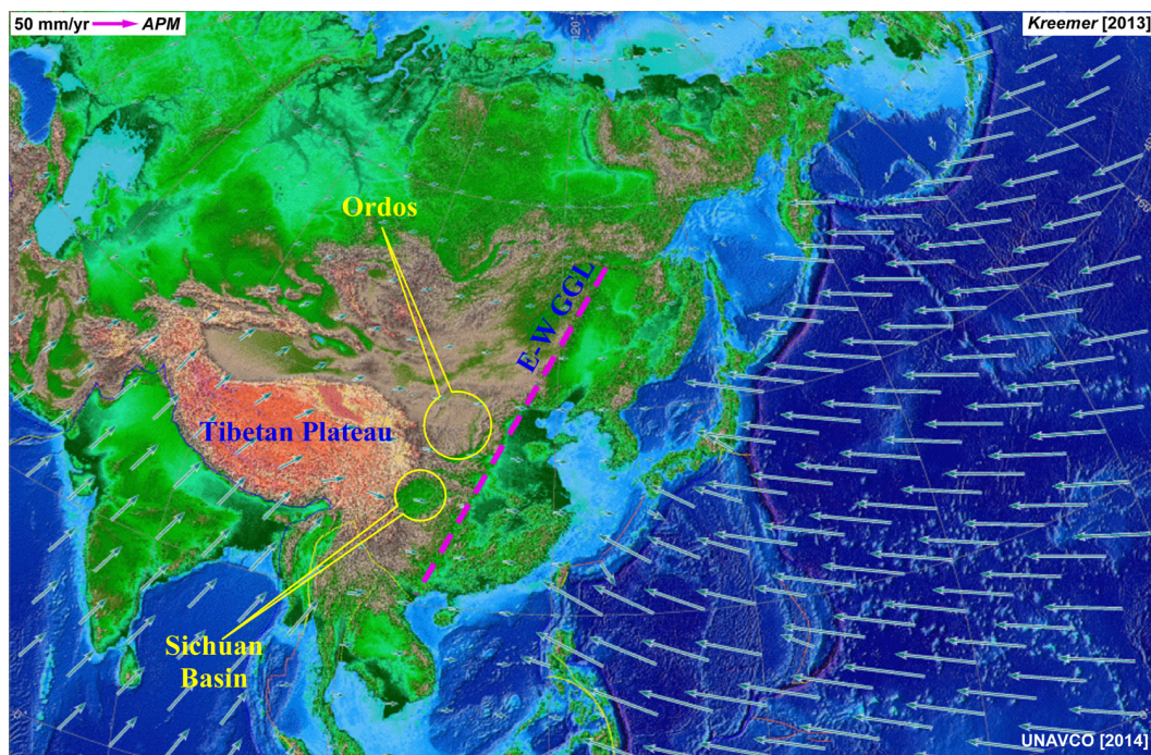
Fig. 11. Portion of the world topographic map emphasizing eastern Asia and western Pacific region with trenches and back-arc basins. Also shown are vectors of plate motion. The southeastward drift of the Chinese continent is the passive response to the trench retreat (see Figs. 8 and 9) of the western Pacific subduction zones. The origins and histories of northern and western Pacific back-arc basins are likely complex, but the mechanism can be readily explained by trench retreat and induced continental drift under internal extension. The pink dashed line is the great gradient line (GGL) marked by contrasting differences in elevation, gravity anomaly, crustal thickness and mantle seismic velocity from high plateaus in the west to hilly plains of eastern China, which is interpreted as the expression of variation in lithospheric thickness from \geq 150 km thick beneath the plateaus in the west to \leq 80 km thick beneath eastern China (Niu 2005b; also see Fig. 10). The Ordos Block and Sichuan Basin west of the GGL are considered the remnant cores of the NCC and Yangtze craton least affected by the lithospheric thinning. Generated from UNAVCO as in Figure 1 ( http://jules.unavco.org/Voyager/GEM_GSRM ).
