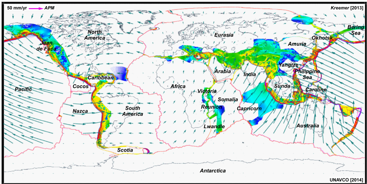
Fig. 16. Global plate tectonics map showing that many plates are not so “rigid” as originally defined (see Fig. 1), but exhibit active deformation of varying nature and degree as indicated by the color-coded locations along convergent margins and in regions within plate interiors. The active deformation has been recognized by means of GPS observations, seismic activities, and active tectonics as well as the need to better fit the global plate motion model (e.g., DeMets et al. 1990; Royer & Gordon 1997; Gordon 1998). These locations and regions are thus better termed as “diffuse plate boundaries” or “diffuse plate boundary zones” (Gordon 1998). As a result, some of the large “rigid” plates become multiple smaller plates. For example, the single large Indo-Australian plate is now considered as made of Indian plate, Australian plate and Capricorn plate because of the recognition of the large “diffuse plate boundary zone” connecting the Java subducting system. Also note the recognition of the Sunda plate, Yangtze plate, Amuria plate and Okhotsk plate as well as the giant diffuse plate boundary zones over much of the continental China all the way to the west along the Himalaya-Alpine Cenozoic orogenic zones from within the original Eurasia plate (Fig. 1). As in Figure 1, also shown are standard plate boundaries and the present-day plate motion vectors using the “sub-asthenosphere” reference frame (APM; from UNAVCO: http://jules.unavco.org/Voyager/GEM_GSRM ).
