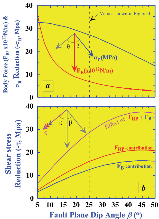
Fig. 5. Calculated forces and stresses as a function of the dip angle \beta of the fault plane across a plate of 95 km thick. a. Potential negative buoyancy forces (or body force; F_B ) at all practical dip angles of 20–45° is similar to or significantly greater than ridge push forces ( \sim 4 \times 10^{12} N/m), which by itself reduces normal stress by \sim 15 to 30 MPa, effectively “opening” the fault plane and creating resistance-free sliding. b. Both F_{RP} and F_B together reduce along-fault plane shear resistance by 25–37 MPa for realistic dip angles (20–45°). This shear-stress reduction is significantly greater than the shear strength of the oceanic lithosphere – only a few MPa (Kanamori & Anderson 1975; Wiens & Stein 1983) and is also greater than the assumed lithosphere shear strength of \sim 10 –20 MPa (McKenzie 1977; Hynes 1982). It should be noted the shear-stress reduction would be > 50 –70 MPa if only the upper elastic portion ( \sim 50 km) is considered, and would be still greater if the effect of water (weakening and lubrication effects) is included. Adapted from Niu et al. (2003).
