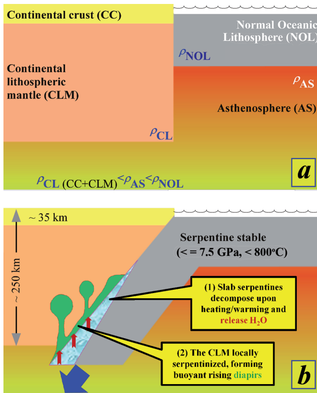
Fig. 6. a. A schematic illustration of density relationships of continental lithosphere (CL), normal oceanic lithosphere (NOL, without considering oceanic plateaus) and asthenosphere (AS). The relative mean densities are estimated to be \rho_{CL} (3.219 g/cc) < \rho_{AS} (3.297 g/cc) < \rho_{NOL} (3.306–3.324 g/cc) with the following assumptions: (1) a 250 km thick cratonic lithosphere with 35 km thick crust; (2) a 95 km thick oceanic lithosphere with 6 km thick crust; (2) room temperature mean density for continental crust \rho_{CC} = 2.800 g/cc, for continental lithospheric mantle \rho_{CLM} = 3.308 g/cc, for ocean crust \rho_{OC} = 3.000 g/cc (3.500 g/cc under eclogite facies during subduction), for oceanic lithospheric mantle \rho_{OLM} = 3.330 , for asthenosphere \rho_{AS} = 3.330 g/cc; (3) mean temperature of 600 °C for both continental and oceanic lithosphere, 1200 °C for asthenosphere; (4) thermal expansion coefficient of 3 \times 10^{-5}/K (see Niu et al. 2003). That is, under realistic conditions, \rho_{NOL}/\rho_{CL} = 1.027 to 1.033 (i.e., 2.7% to 3.3% denser), and \rho_{NOL}/\rho_{AS} = 1.003 to 1.008 (i.e., 0.3% to 0.7% denser), which are physically significant (see Niu and Batiza, 1991a,b). b. It is well known that the oceanic upper mantle lithosphere beneath the crust is highly serpentinized (Dick 1989; Niu & Hekinian 1997; Niu 2004). It is also known experimentally that serpentines can be stable up to 7.5 GPa at T \leq 800 °C (Ulmer & Trommsdorff 1995; Williams & Hemley 2001; also see Fig. 14). Hence, it shows the possibility that serpentines of the subducting oceanic lithosphere beneath the thickened cratonic lithosphere can become unstable under heating/warming and thus decompose and lose the water into the overlying continental lithospheric root, which can then cause serpentinization within it under the conditions of P \leq 7.5 GPa and T \leq 750 °C. The serpentines can form and rise as diapirs, carrying its ambient harzburgitic rock fragments and high pressure minerals like diamonds seen in some “supra-subduction ophiolites” including the Luobusha chromitite mine in southern Tibet (Bai et al. 1993; Robinson et al. 2004; Yang et al. 2007, 2014; Dobrzhinetskaya et al. 2009).
