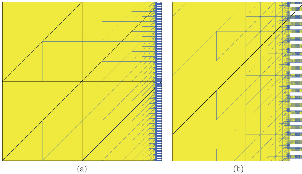
FIG. 9.1. Example 1: (a) Initial CFE mesh. The color blue (right-hand edge) denotes elements present in the fine level mesh (which consists of 20160 triangular elements); elements plotted in black form the coarse level mesh (containing eight elements); finally, the domain \Omega is shown in yellow (gray). (b) Zoom of (a).
