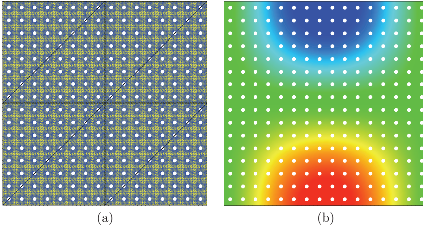
FIG. 9.2. Example 2: (a) Initial CFE mesh. Fine level mesh consisting of 85500 triangular elements and coarse level mesh (solid black line) containing eight elements. (b) Analytical solution.
