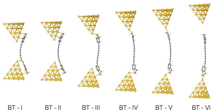
Figure 7. Examples of junction evolution of oligoene derivatives BT4 showing key configurations.
