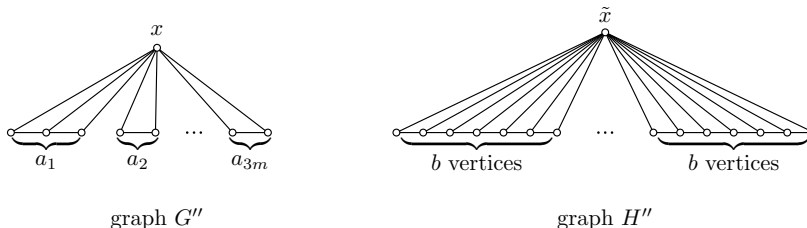
Fig. 4. A schematic illustration of the graphs G'' and H'' that are constructed from a given instance (A, b) of 3-PARTITION in the proof of statement (iii) in Theorem 1.
