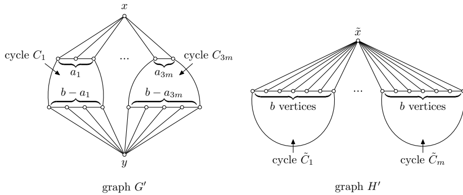
Fig. 3. A schematic illustration of the graphs G' and H' that are constructed from a given instance (A, b) of 3-PARTITION in the proof of statement (ii) in Theorem 1.
