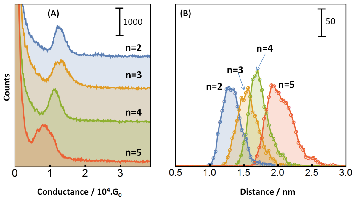
Figure 1: I(s) conductance (A) and break-off distance (B) histograms recorded for the series of oligynes 2, 3, 4, 5 in PC. Conductance histograms have been offset vertically for clarity.
