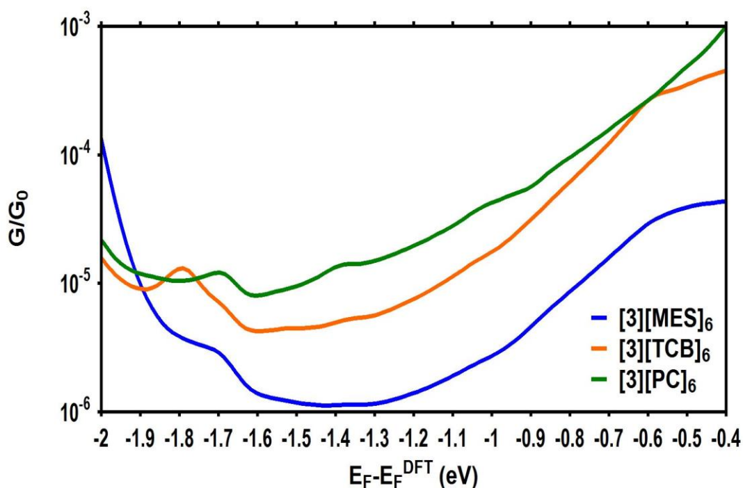
Figure 9: The room-temperature conductances as a function of the Fermi energy for 3 in mesitylene (MES), trichlorobenzene (TCB) and propylene carbonate (PC).
