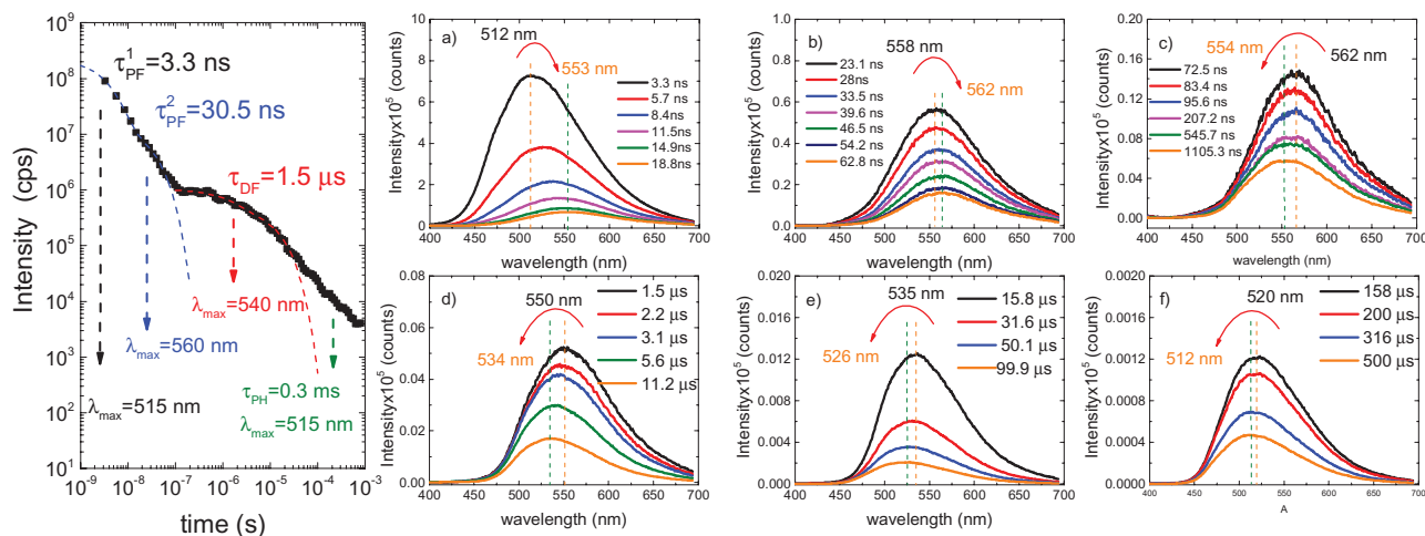
Figure 7. Emission decay and time resolved spectra obtained at different delay times for DPTZ-DBTO2 dispersed in zeonex at RT. a) ^1\text{CT} , prompt fluorescence emission spectra showing a contribution from ^1\text{LE} fluorescence at very early times (less than 3 ns). b) ^1\text{CT} fluorescence, possibly also containing a DF contribution, emitting around 560 nm between 23 and 63 ns. c) From 73 ns to 1.1 \mu\text{s} , the ^1\text{CT} emission is dominated by delayed fluorescence, and at later times the contribution of the far more slowly decaying ^3\text{LE} phosphorescence emerges, causing a blueshift in the emission peak. d) ^1\text{CT} delayed fluorescence, decaying from 1.5 to 11.2 \mu\text{s} . The relatively stronger contribution of the underlying ^3\text{LE} phosphorescence causes the emission maxima to effectively shift to shorter wavelengths. e, f) ^1\text{CT} delayed fluorescence, decaying from 15.8 to 500 \mu\text{s} , showing a continuous blueshift in the maxima toward 505 nm where the ^3\text{LE} phosphorescence peaks.
