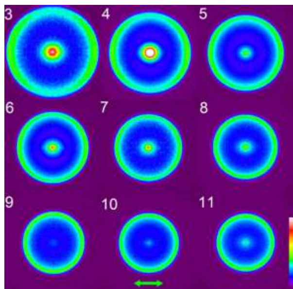
Figure 7: Photoelectron images of {}^-\text{O}_2\text{C}(\text{CH}_2)_m\text{CO}_2^- for 3 \leq m \leq 11 taken at 3.496 eV. The laser polarisation is indicated and is horizontal. Taken from Ref. 36 with permission from American Physical Society.
