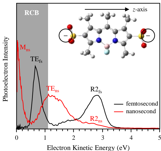
Figure 6: Photoelectron spectra of pyromethene 556 dianion taken at 2.38 eV with a nanosecond (ns) laser and at 2.43 eV with a femtosecond (fs) laser. ‡ Grey shading indicates the kinetic energy cut-off due to the RCB. Labels indicate the following: R2, two-photon resonance enhanced detachment; TE, tunnelling emission; and M, emission from the monoanion. Adapted from Ref. 44 and 68, with permission from American Chemical Society and American Institute of Physics.
