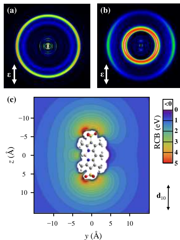
Figure 8: Photoelectron imaging of pyromethene 556 dianions taken at (a) 4.66 eV and (b) 2.43 eV, where the latter energy is resonant with the S_1 \leftarrow S_0 transition. (c) The calculated RCB in the plane of the molecule, where \mathbf{d}_{10} indicates the direction of the transition dipole moment. The laser polarisations are indicated in (a) and (b). Adapted from Ref. 44 and 68, with permission from American Chemical Society and American Institute of Physics.
