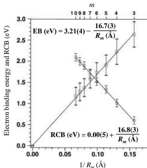
Figure 3: Dependence of the RCB height and electron binding energy as a function of the Coulomb repulsion ( 1/R_m ) between the negative charges in ^-O_2C(CH_2)_mCO_2^- . Adapted from Ref. 18, with permission from American Physical Society.
