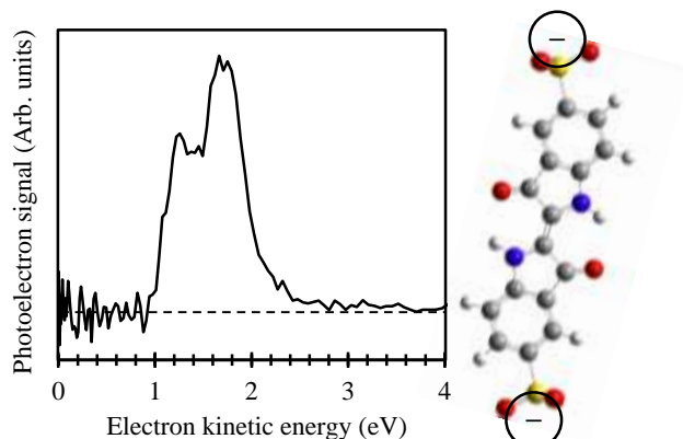
Figure 2: Photoelectron spectrum of the indigo carmine dianion (shown) taken at 4.66 eV, which highlights the presence of the cut-off at eKE \sim 1.1 eV, below which no photoelectrons are emitted. Adapted from Ref. 21, with permission of the PCCP Owner Societies.
