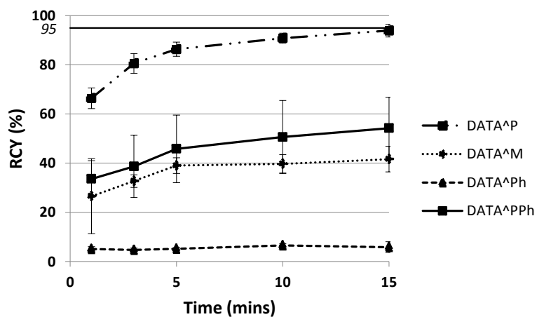
Figure 8 Radiolabelling Time dependence of radiolabelling at pH 6 (23 °C) for DATA M (7 nmol), DATA P (7 nmol), DATA Ph (5 nmol) and DATA PPh (7 nmol).
