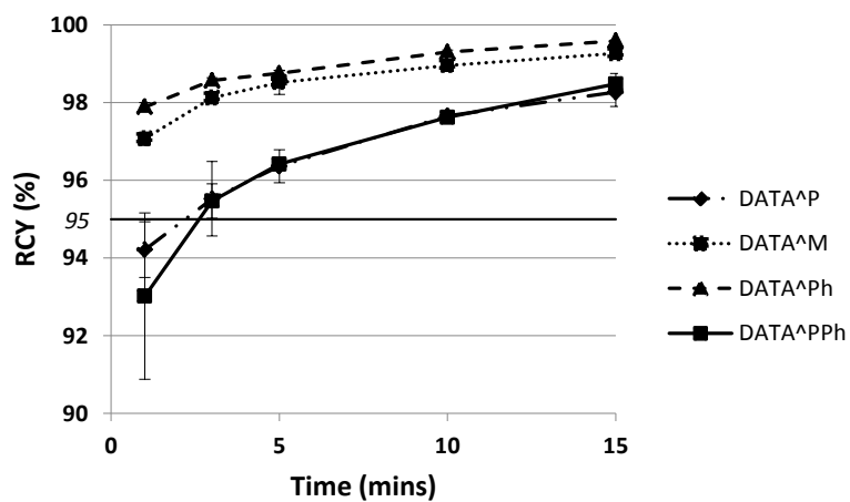
Figure 7 Radiolabelling Time dependence of radiolabelling kinetics at pH 5 (23 °C) for DATA M (7 nmol), DATA P (7 nmol), DATA Ph (5 nmol) and DATA PPh (7 nmol).
