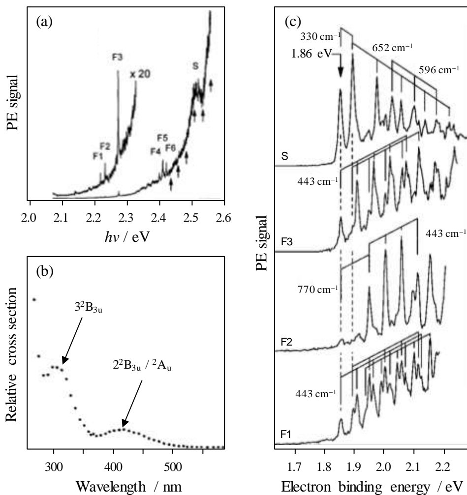
Figure 6: Photodetachment photoelectron spectra of pBQ^- . (a) and (b) show high- and low-resolution total photoelectron yield spectra. The sharp features in (a) arise from Feshbach resonances (F1 – F6) and a broad feature from the origin of the ^2A_u shape resonance (S); the low-resolution spectrum shows the relevant resonances over the first few eV of the continuum. Photoelectron spectra in (b) were taken at photon energies that are resonant with the resonances identified in (a). Panels (a) and (c) are adapted from reference 87 and (b) from reference 88.
