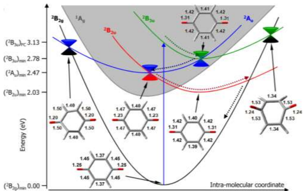
Figure 10: Calculated critical points in the pBQ - . A conical intersection between the 2^2B_{3u} and 2^2A_u resonances was located near the minimum of the 2^2B_{3u} potential energy surface, which provides an efficient pathway to internally convert to 2^2A_u . Other conical intersections leading to the ground electronic state are identified. Reproduced from reference 96.
