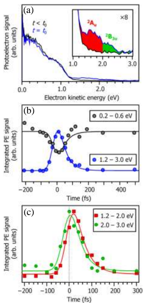
Figure 9: Time-resolved photoelectron spectroscopy of pBQ - following excitation at h\nu = 3.10 eV ( 2^2B_{3u} resonance). Two representative photoelectron spectra are shown in (a) with probe arriving before the pump ( t < t_0 ) and both pump and probe temporally overlapped ( t = t_0 ). The inset shows an expanded view of the high-energy time-resolved feature, which can be divided into 2^2B_{3u} and 2^2A_u contributions. Integral photoelectron contributions are given in (b) and (c). In (b), the two integration regions represent the pump-probe appearance signal and depletion signal. In (c), the integration regions represent the signal arising from the 2^2B_{3u} and 2^2A_u resonances, as indicated in (a). Reproduced from reference 96.
