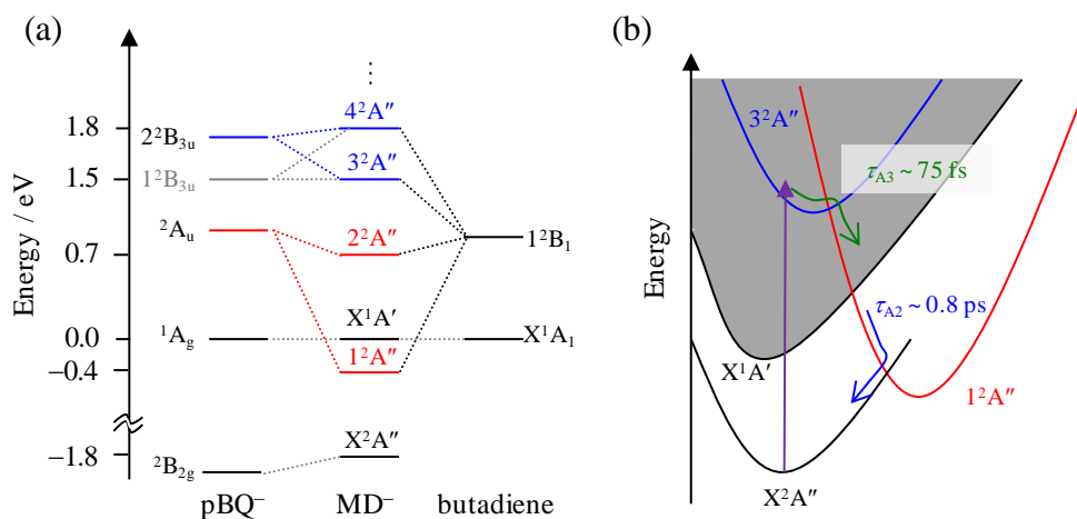
Figure 13: (a) Correlation diagram of ground and excited electronic state energetics of \text{MD}^- , \text{pBQ}^- , and cis -butadiene. A schematic summary of the excited state dynamics of \text{MD}^- is given in (b), showing the initially excited 3^2\text{A}'' resonance internally converts to the bound electronic 1^2\text{A}'' state in \sim 75 fs., which then internally converts to the ground electronic state on a slower \sim 800 fs timescale. The ground electronic state detaches the electrons as thermionic emission.
