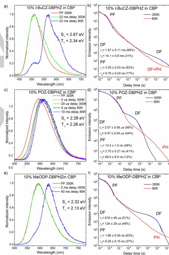
Figure 3. PF, DF, and PH spectra of 10 wt% a) t-BuCZ-DBPHZ , c) POZ-DBPHZ , and e) MeODP-DBPHZ in CBP blended films; Transient decays of 10 wt% b) t-BuCZ-DBPHZ , d) POZ-DBPHZ , and f) MeODP-DBPHZ in CBP films measured at 300K and 80K.
