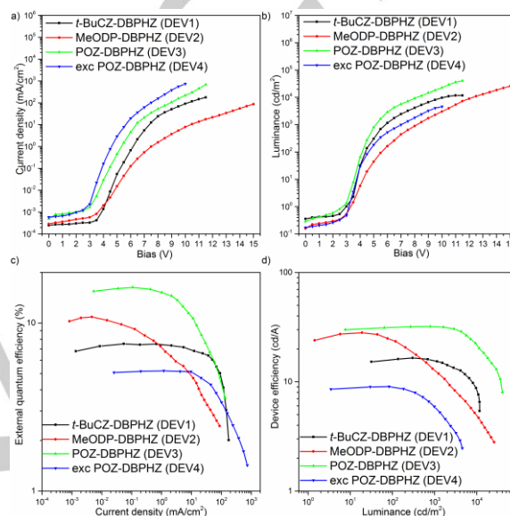
Figure 5. Device characteristic of DEV 1–4.
