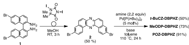
Scheme 1. Synthetic route to U-shaped D-A-D compounds.
