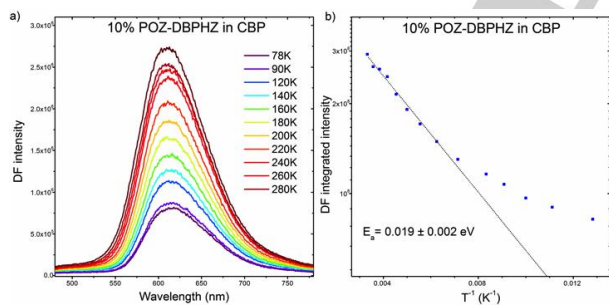
Figure 4. Temperature dependence of DF in 10 wt% POZ-DBPHZ :CBP blended film: a) spectra and b) plot of DF integrated intensity vs. temperature with calculated activation energy.
