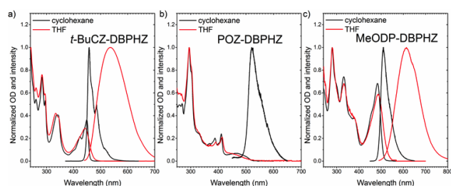
Figure 2. Absorption and PL spectra of a) t-BuCZ-DBPHZ , b) POZ-DBPHZ , and c) MeODP-DBPHZ solutions of specified solvent (concentration: 10^{-4} M).
