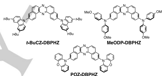
Figure 1. Structures of the investigated DBPHZs.
