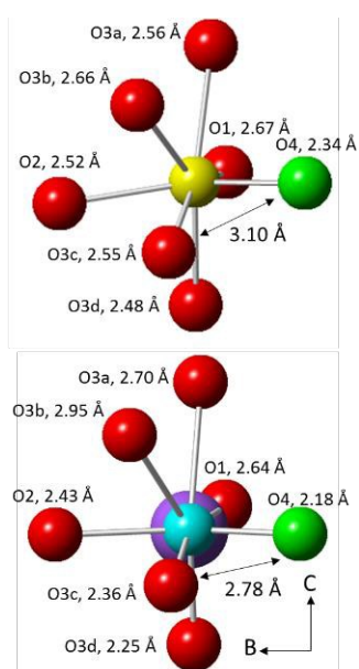
Figure 5: Comparison of the local environments around an A2 La site in \text{La}_{10}\text{Ge}_6\text{O}_{27} (top) and an A2 Bi site in \text{Bi}_2\text{La}_8\text{Ge}_6\text{O}_{27} (bottom). The yellow atom is La, blue is Bi, green is O4 and red are other O atoms. The purple region indicates the orientation of the Bi lone pair. 52
