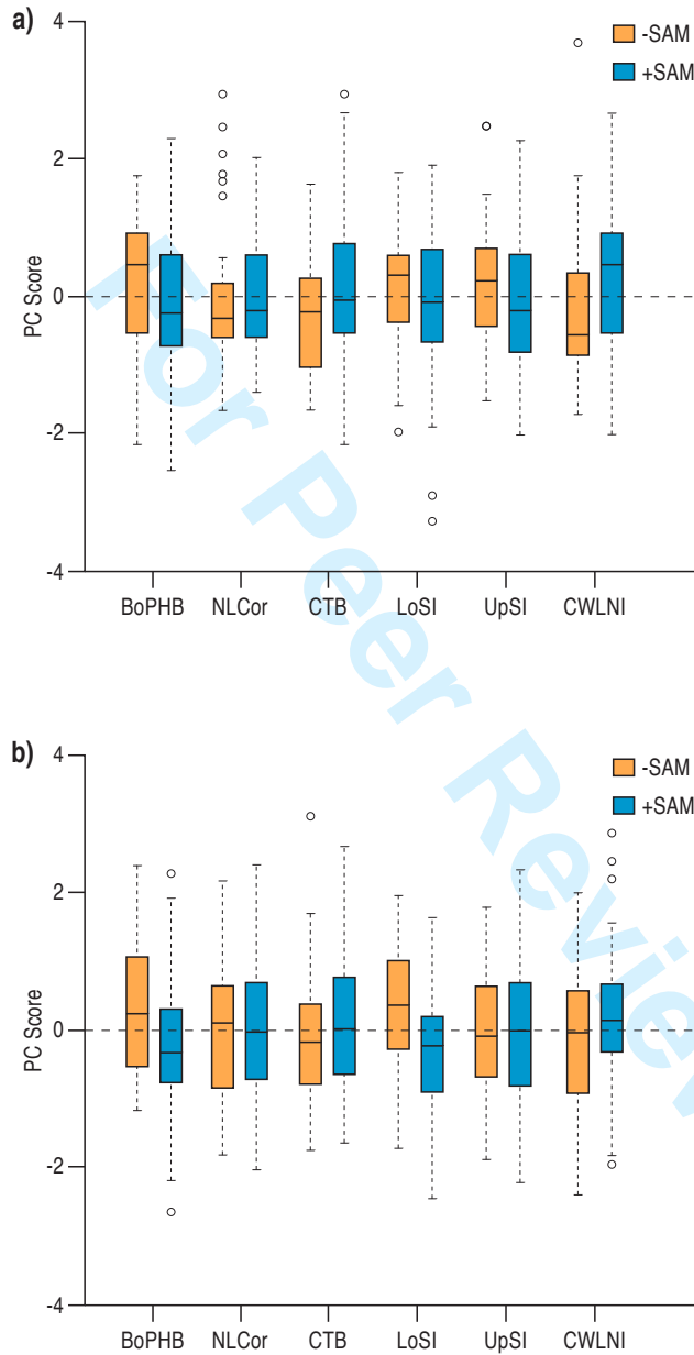
Figure 5: Principal component score (as a proxy of river flow) distribution by region for positive (+SAM) and negative (-SAM) phases of SAM for (a) DJF and (b) JJA as revealed by the circulation to environment approach. The form of the box plots is as described for Figure 4.
