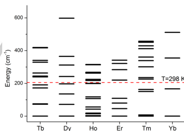
Figure 2. Energy splitting of the ground terms of [Ln.L 1 ] due to the ligand field, computed by CASSCF/SOC-RASSI as implemented in MOLCAS 8.0. Calculations demonstrate that the LF splitting is larger than room temperature kT , indicating that Bleaney's approximation is not valid.
