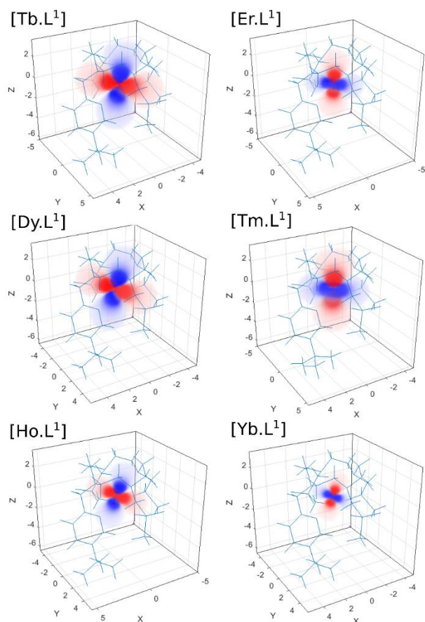
Figure 1. Pseudocontact shift fields for [Ln.L 1 ] complexes reconstructed by Spinach 91 using the best-fit magnetic susceptibility tensor. Positive PCS is shown in red, negative - in blue, transparency indicates the absolute value normalized for all complexes (see the ESI for further information).
