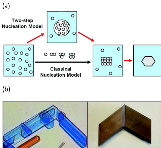
Figure 6. (a) Classical vs. non-classical nucleation models (reproduced with permission from reference 65) (b) Oriented attachment in gypsum crystals (reproduced with permission from reference 66)
