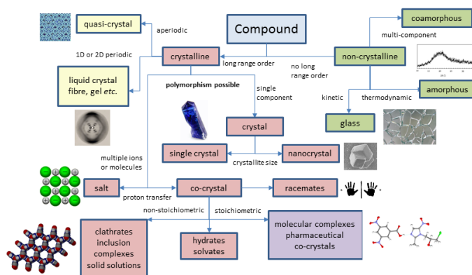
Figure 2. The scope of molecular materials (adapted from ref. 16).
