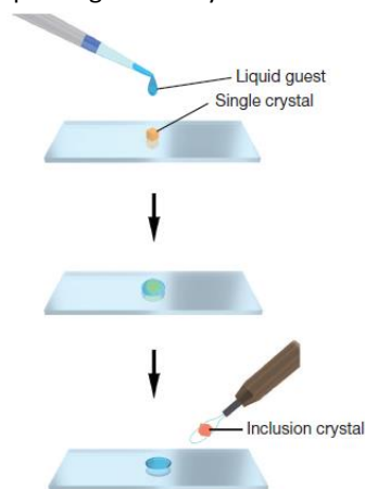
Figure 4. Preparation of a guest included network complex: a single piece of crystalline sponge is treated for 2 d (possibly under sealed conditions for volatile liquids) with a drop of a liquid guest and subjected to X-ray data collection (reproduced with permission from reference 31).
