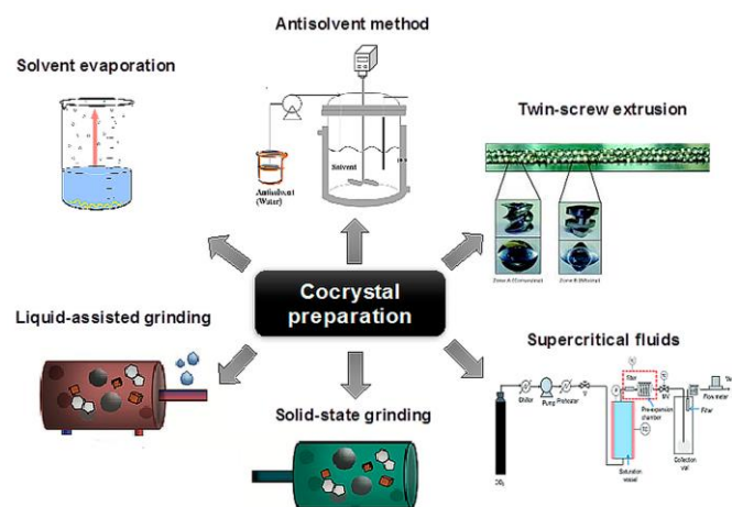
Figure 3. Methods for co-crystal preparation (reproduced with permission from ref 18).
