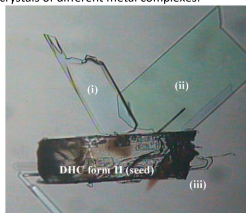
Figure 7. Crystals of the computationally predicted catemeric carbamazepine Form V (I – iii) growing on a catemeric dihydrocarbamazepine form II seed crystal (reproduced with permission from ref. 86 ).
