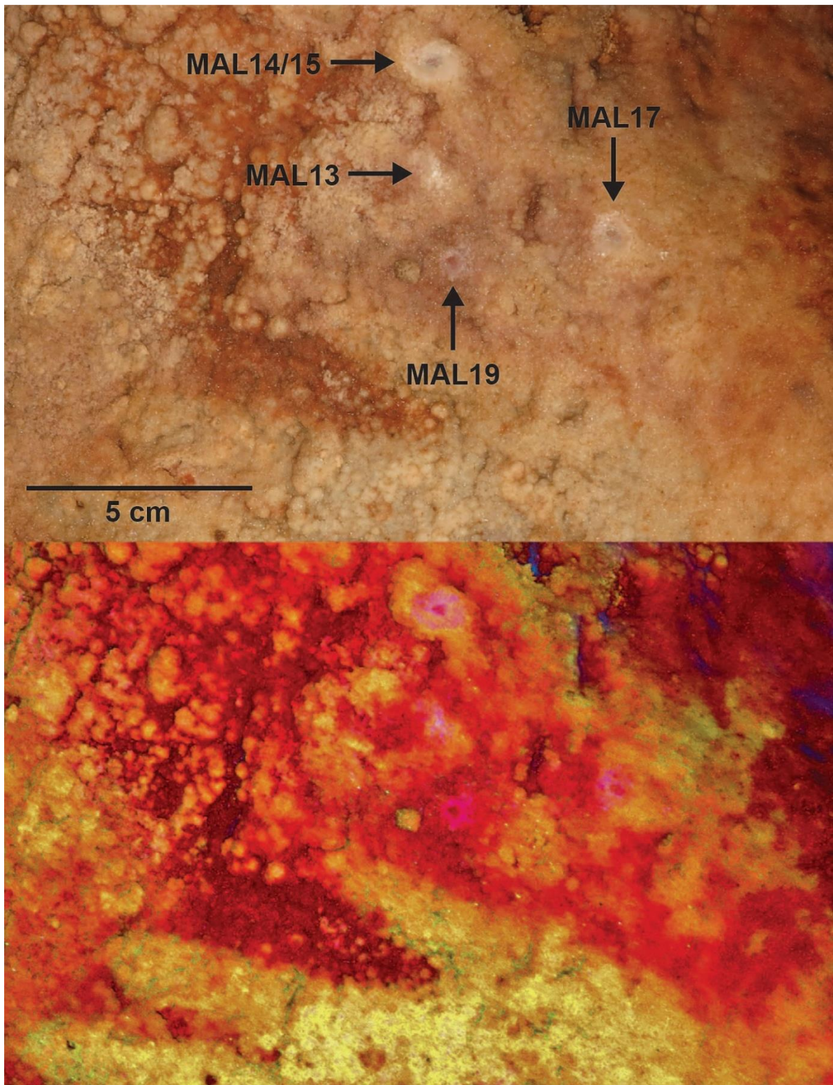
Fig. S16. Sampling of hand stencil GS3b, Maltravieso. The upper picture shows the original photo with labelled sample locations, the lower is the same picture after application of DStretch (Correlation CRGB 15 %, auto contrast). Pigment is clearly visible in the valleys and cracks between carbonate growths.
