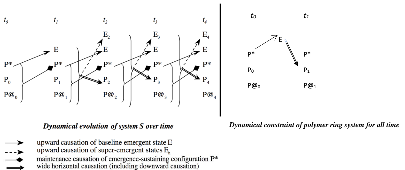
Figure 5. Comparison of the emergent variable scheme of O'Connor and Wong (2005) (left) with the description, in the same notation, of the polymer ring system example (right). P* denotes a complex physical configuration of a system S at time t 0 . P 0 comprises 'the remaining aspect of S's physical state at time t 0 '. P@ 0 are the environmental factors outside S that bear upon its evolution. In the polymer system a single set of emergent (topological) variables arises immediately from the configuration of the system, whose values co-determine all future microscopic configurations P 1 of the fluid.
