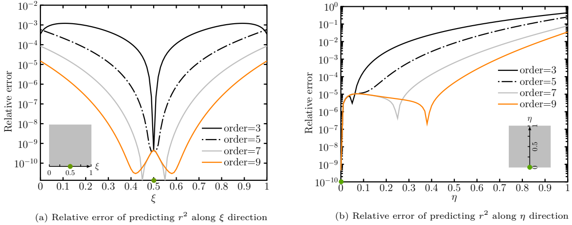
Figure 13: Relative error of predicting r^2 when the projection point lies at a boundary of an element
