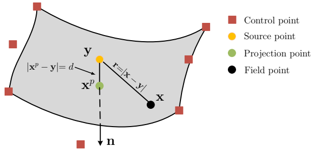
Figure 2: Minimum distance d to the element when \mathbf{x}^p \in \Gamma_e
