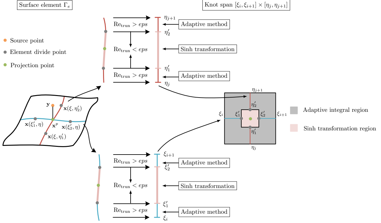
Figure 14: Element division and choice of integral method on a surface isogeometric element
