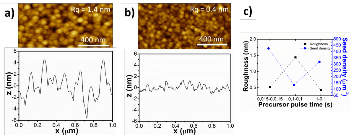
11 Figure 5. AFM micrographs and line profiles of samples (a) S4 and (b) S5 in which the influence of the 12 precursors pulse time was studied. (c) Comparison of roughness values and seed density 13 obtained from the AFM images for S3, S4 and S5.
