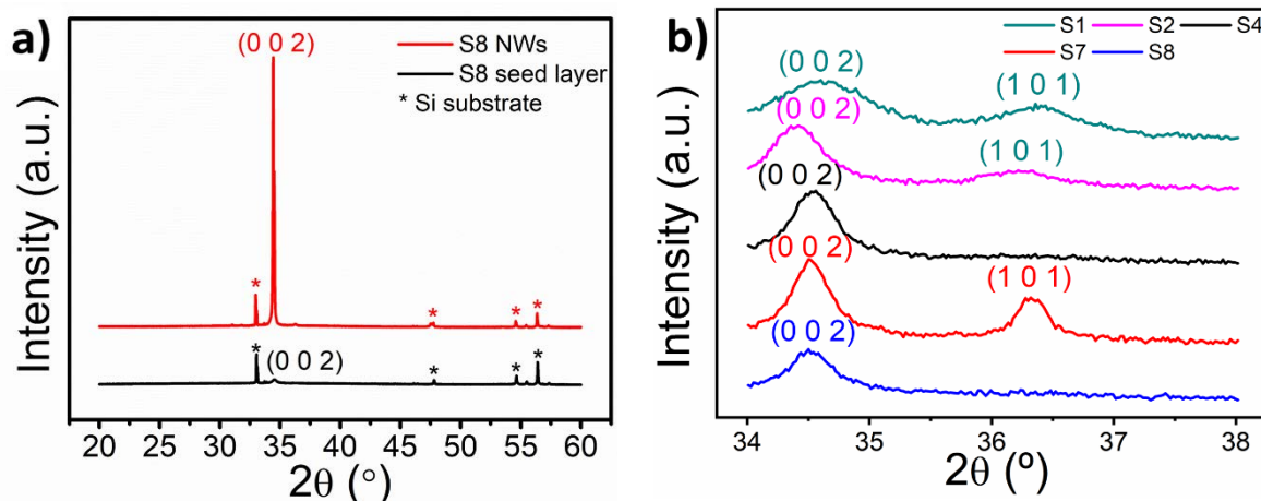
1 Figure 2. XRD spectra of a comparison between seed layer and NWs grown on it (a) and detail of the 2 (0 0 2) peak for five different seed layers (b).
