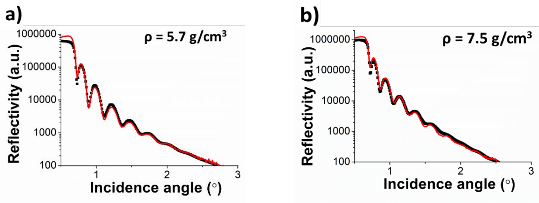
2 Figure 6. X-ray reflectivity spectra obtained for seed layers (a) S4 and (b) S5 from the best-fitting seed 3 layer density values. Black symbols show experimental data while red lines indicate the best 4 fitting simulation obtained for the data.
