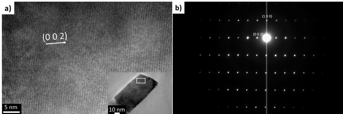
7 Figure 12. (a) HRTEM image of a ZnO NW and (b) the correspondent diffraction pattern.
