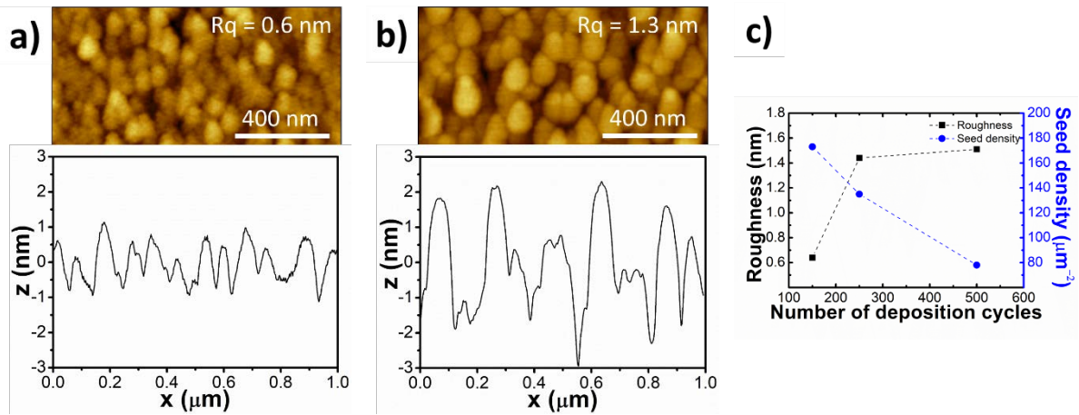
1 Figure 8. AFM micrographs and line profiles of (a) S6 and (b) S7 in which the influence of the number 2 of deposition cycles was studied. (c) Comparison of roughness values and seed density 3 obtained from the AFM images.
