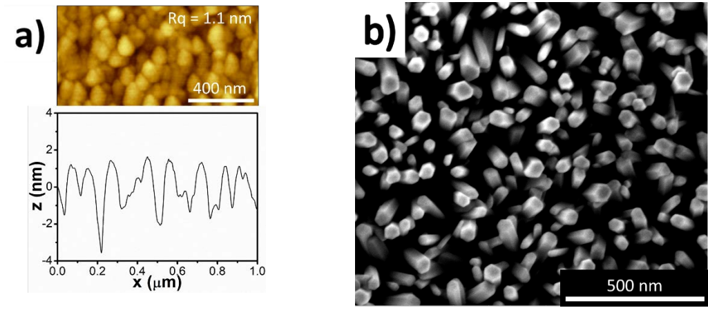
4 Figure 10. (a) AFM micrograph and line profile of S8 in which the influence of the purge times was 5 studied. (b) FESEM imaging of S8.
