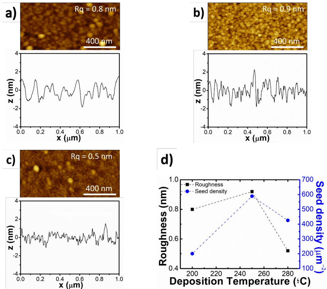
5 Figure 3. AFM micrographs and line profiles of (a) S1, (b) S2 and (c) S3, in which the temperature 6 influence was studied. (d) Comparison of roughness values and seed density obtained from 7 the AFM images.
