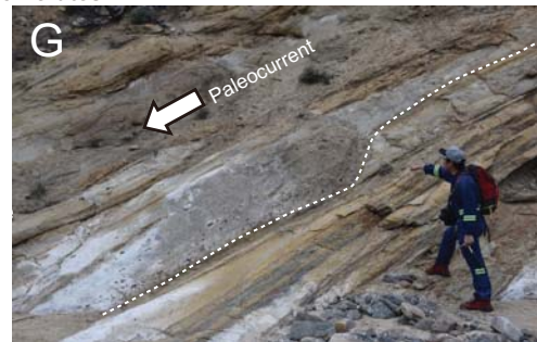
A step-like erosion surface
