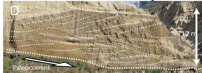
Consistent backsets in conglomerates
