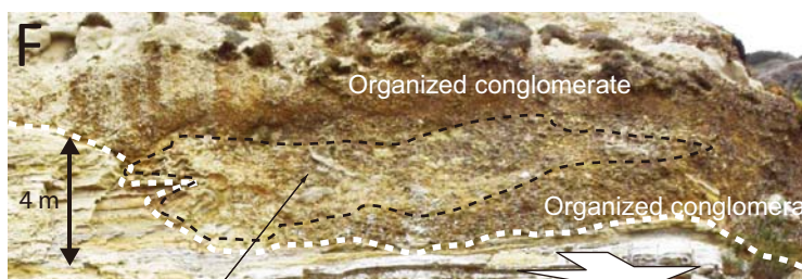
Normal graded conglomerates
