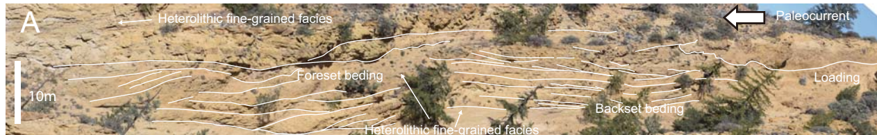
Amalgamated erosively bound gravel lenses with foreset and backset bedding
