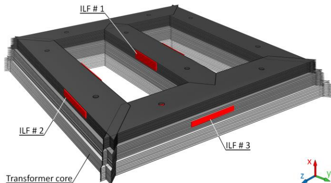
Fig 1 A three-phase three-limb transformer core with ILF in the limbs and yoke
