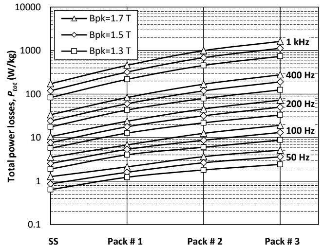
Fig 7 Total power loss of the test samples at different magnetising frequencies and peak flux densities
