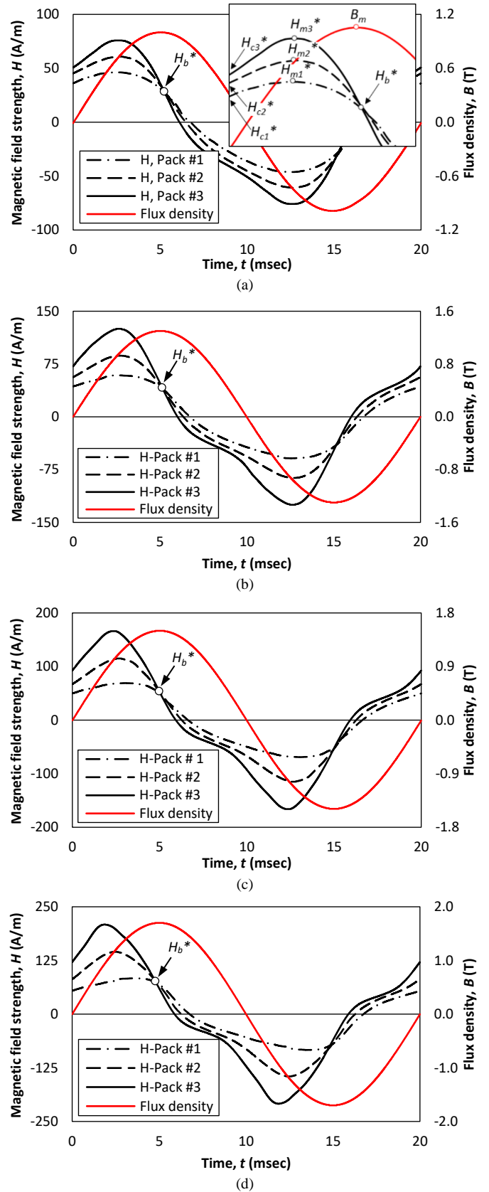
Fig 10 Instantaneous wave shapes of magnetic field strength H(t) of the test samples for one magnetising cycle at frequency of 50 Hz and peak flux densities of (a) B_{pk}=1.0 T, (b) B_{pk}=1.3 T (c) B_{pk}=1.5 T and (d) B_{pk}=1.7 T
