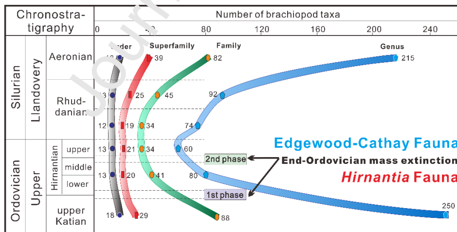
Fig. 19. Taxonomic changes in brachiopod diversity through the Ordovician and Silurian transition.
