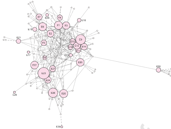
Fig. 16. Network analysis showing the connectivity for occurrences of genera and a close relationship between the Edgewood Fauna (E1–E21) and the Cathay Fauna (E22–E29). Size of node indicates the diversity of the collection that represented. Although many endemic taxa made the Cathay Fauna relatively independent, the clear boundary was not detected between the two faunas. The late Hirnantian deep water associations (E8, E28) are not included. E30 (South Africa) may presumably represent a high latitude brachiopod province in the late Hirnantian and early Rhuddanian.
