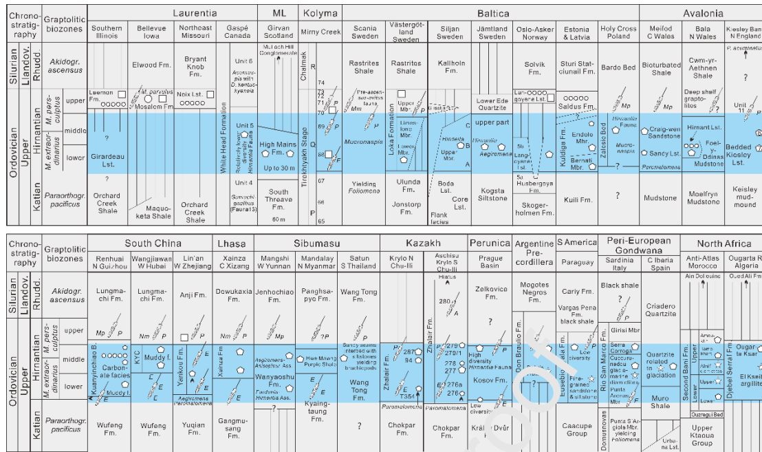
Fig. 4. Global correlation chart of biostratigraphy and lithostratigraphy across the Ordovician and Silurian boundary. Laurentia: Illinois, Iowa, and Missouri (Barnes and Bergström, 1988; Elias and Young, 1998; Loydell et al. , 2002; Stott and Jin, 2007; Bergström et al. , 2012b); Percé, Québec (Lespérance, 1988). Marginal Laurentia: Girvan, Scotland (Harper, 1981, 2006). Baltica: Jämtland (Dahlqvist et al. , 2010), Scania (Koren et al. , 2005), Siljan (Suzuki et al. , 2009; Ebbestad et al. , 2015; Kröger et al. , 2015), and Västergötland (Eversström, 1968; Bergström and Bergström, 1996), Sweden; Oslo–Asker Region, Norway (Cocks, 1982; Brenchley and Cocks, 1982; Bockelie et al. , 2017); Estonia–Latvia (Harper and Hints, 2016; Hints and Harper, 2015); Holy Cross Mountains, Poland (Masiak et al. , 2003). Avalonia: Meifod, C Wales (Brenchley et al. , 2006; Schmitz and Bergström, 2007; Blackett et al. , 2009), Bala, N Wales (Temple, 1965; Brenchley and Cullen, 1984; Vandenbroucke et al. , 2008); Westmorland, N England (Temple, 1968; Wright, 1985, 1988; Cocks, 2008), UK. South China (Chen et al. , 2000; Rong et al. , 2002, 2013, 2018; Zhang et al. , 2007). Lhasa: Xainza, C Xizang (Rong and Xu, 1987). Sibumasu: Mangshi, western Yunnan (Fang et al. , 2018; Huang et al. , 2020a, c); Mandalay, Myanmar (Chen et al. , 2020; Rong et al. , 2020); Satun, S Thailand (Cocks and Fortey, 1997). Kazakh: Chu–Ili (Nikitin et al. , 1980). Perunica: Prague Basin, Bohemia (Štorch and Loydell, 1996; Štorch et al. , 1989, 2019). Argentine Precordillera (Sánchez et al. , 1991; Rickards et al. , 1996; Benedetto, 2003; Halpern et al. , 2014). South America: Bolivia and Paraguay (Benedetto et al. , 2013, 2014). European peri–Gondwana: Sardinia, Italy (Štorch and Leone, 2003); Central Iberia, Spain (Villas et al. , 1999; Sutcliffe et al. , 2001). North Africa: Anti–Atlas, Morocco (Ougarf, 2001); Ougarf, Algeria (Ougarf, 2001); Ougarf, Algeria (Ougarf, 2001).
