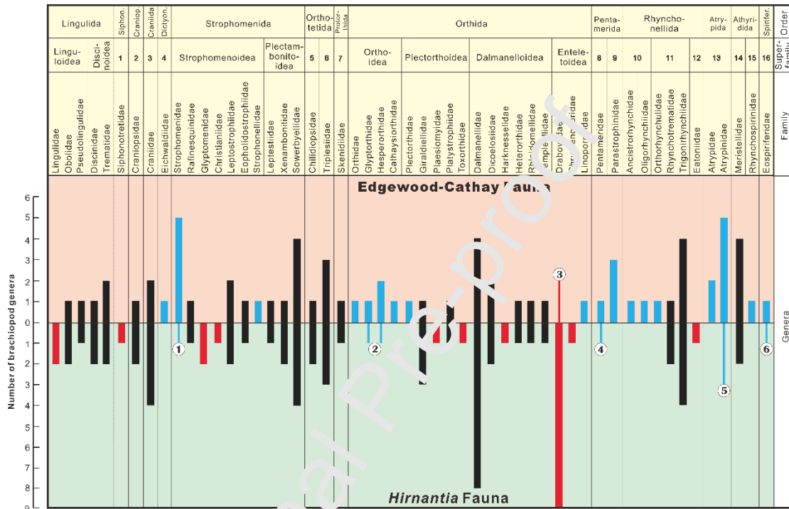
Fig. 18. Showing number of brachiopod genera in each family occurring in the Hirnantia Fauna and the Edgewood-Cathay Fauna. Numbered superfamilies include: 1 Siphonotreta, 2 Cranioidea, 3 Cranioidea, 4 Eichwaldioidea, 5 Chilidiopsidae, 6 Triplesioidea, 7 Skenidioidea, 8 Pentamerida, 9 Camerelloidea, 10 Ancistrothyridae, 11 Rhynchotrematoidea, 12 Uncinuloidea, 13 Atrypidae, 14 Meristelloidea, 15 Athyrida, 16 Cyrtioidea. Blue bar representing those only or mostly known in the Edgewood-Cathay Fauna; red bar representing those only or mostly known in the Hirnantia Fauna; black bar occurring in the both faunas. Circles: (1) No strophomenids in the Hirnantia Fauna with the exception of Titanomena (Bergström, 1968); orthoids (2), pentamerides (4) and spiriferides (6) very rarely and atrypides (5) rarely known in the Hirnantia Fauna; (3) draboviids rarely discovered in the
