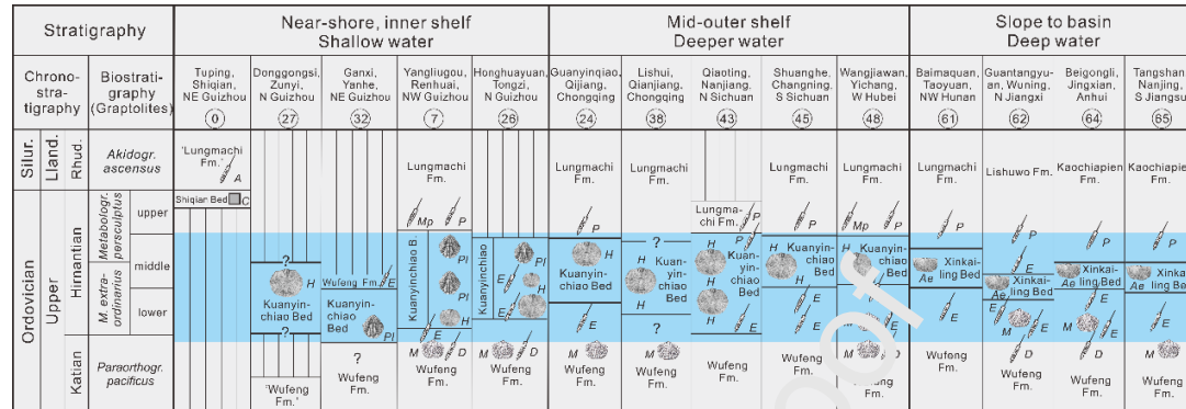
Fig. 3. Correlation chart of the Ordovician–Silurian boundary successions at selected sections in South China, including the successions of inner shelf, mid–outer shelf, and slope to basin, showing various stratigraphic positions of the Hirnantia Fauna-bearing beds. The Kuanyinchiao Bed, yielding near-shore, shallow water, low diversity communities of the Hirnantia Fauna, characterized by the Dalmanella – Plectothyrella Community and the relatives lacking Hirnantia and Kinnella in carbonate facies (BA 2) (PI), and mid–outer shelf, relatively deeper water, moderate to high diversity Hirnantia Fauna in mudstone and siltstone (BA 3) (H). The Xinkailing Bed, containing deep water, low diversity Hirnantia Fauna (Ae), typified by the dominance of Aegiromena lacking Hirnantia and Kinnella . This figure shows the occurrences of the graptolites, Diceratograptus mirus (D), Metabolograptus extraordinarius (E), M. persculptus (P), M. parvulus (Mp), and A. ascensus (A) (Li et al. , 1984; Yu et al. , 1984; Chen et al. , 2000, 2005; Rong et al. , 2002), associated with occurrences of the brachiopods Manosia (M) (Rong and Huang, 2019) and Cathaysiorthis (C) (Rong et al. , 2013). Numbers are as in Fig. 2.
