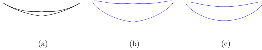
Figure 21: Deformed shapes for circular arc crack ( 2\theta = 60^\circ ) considering the contribution from (a) the NURBS basis functions and (b) the enrichment term. (c) Final deformed shape for curved crack, given by the superposition of solutions from (a) and (b). Enriched NURBS are depicted in blue (please refer to the coloured version).
