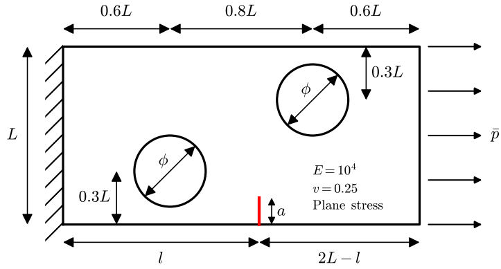
Figure 28: Tensioned rectangular plate with two holes and an edge crack.
