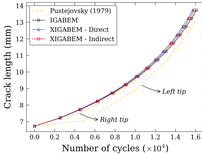
Figure 24: Crack length evolution with number of load cycles. The solutions obtained experimentally by Pustejovsky [75] are also provided.
