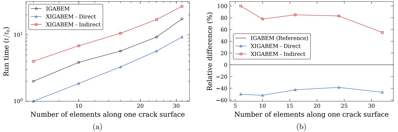
Figure 18: (a) Variation of execution time with crack mesh refinement. The values are normalised by t_0 = 10.9 ms, which is the smallest time observed and corresponds to the run time of the direct XIGABEM for the coarsest discretisation. (b) Relative differences between run times considering the indirect IGABEM results as reference.
