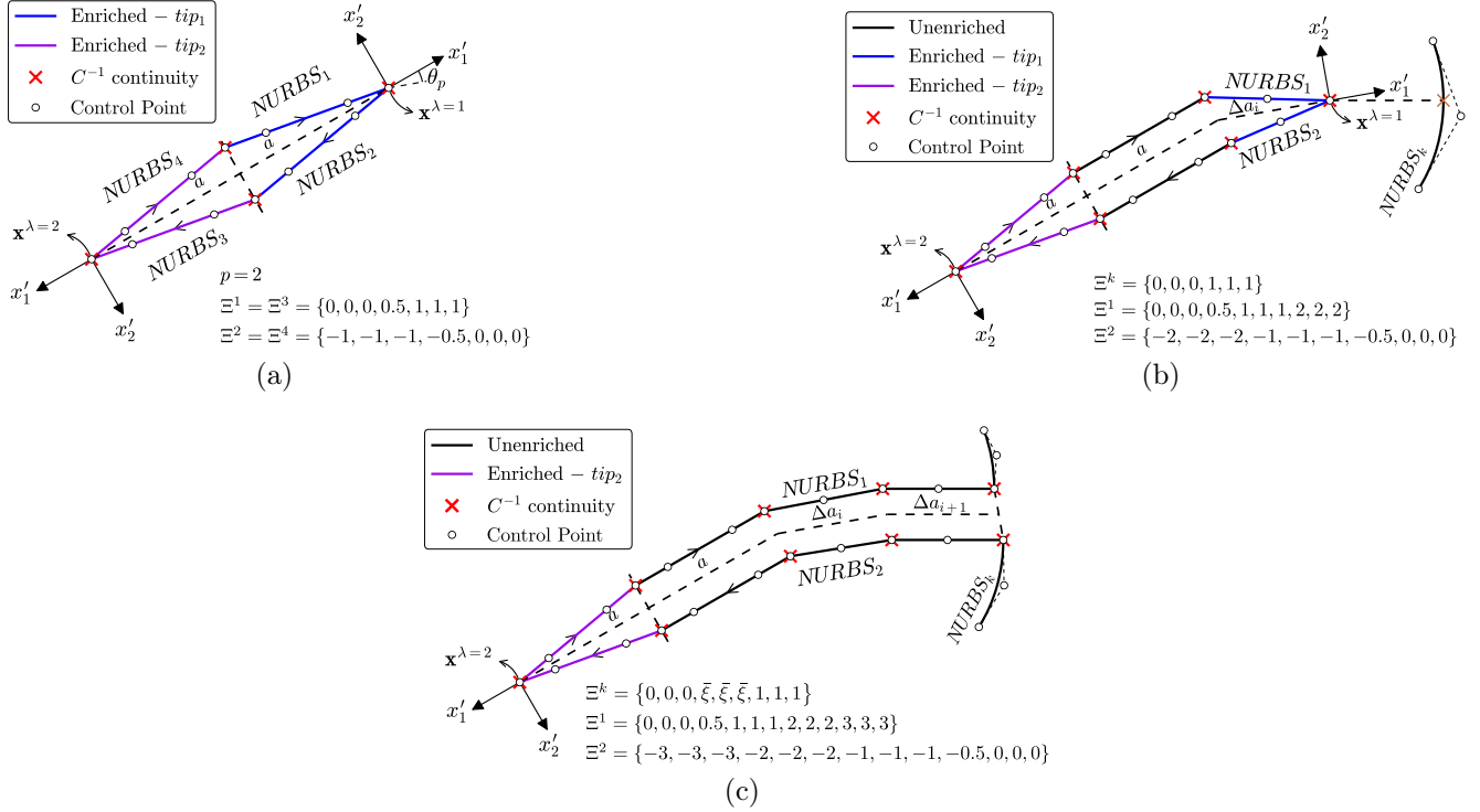
Figure 6: (a) Representation of enriched NURBS for an interior crack. In this example, the basis functions are assumed with order p = 2 and each NURBS is initially discretised into two elements (two knot spans in the knot vector). (b) NURBS and their enriched parts after a crack tip propagation. Each new NURBS segment is discretised into one element (one additional knot span in the knot vector) and the multiplicity for the knot at the former tip is kept equals to p + 1 . (c) Intersection between the crack tip \lambda = 1 with another NURBS, which is initially discretised into one element in the illustrative example. In this case, the respective crack NURBS no longer benefit from enrichment. Besides, the crossed NURBS is made discontinuous at the intersection by increasing the multiplicity of the intersection knot \bar{\xi} to p + 1 through successive knot insertions. After this processed, the intersected NURBS becomes discretised into two elements, each defined by independent control points.
