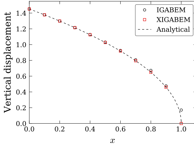
Figure 9: Deformed shape for the upper crack surface determined by IGABEM and XIGABEM.
