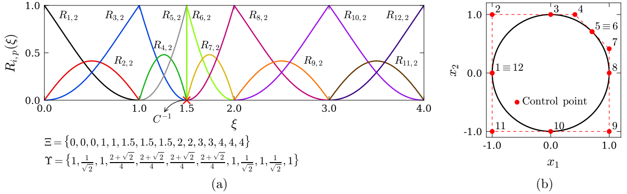
Figure 2: (a) NURBS basis functions after p + 1 knot insertions at \bar{\xi} = 1.5 . (b) Representation of the NURBS curve and new control points positions. Control points 5 and 6 end up in the same position after the successive knot insertions; however, the NURBS curve may be discontinuous at this point if the coincident control points are moved to different locations.
