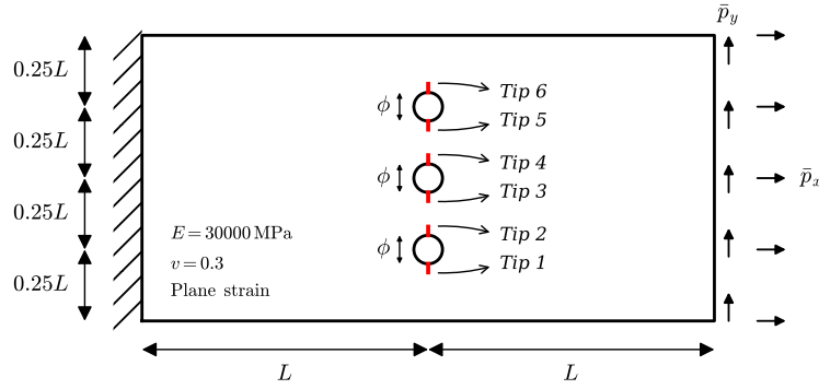
Figure 32: Perforated panel containing multiple cracks.
