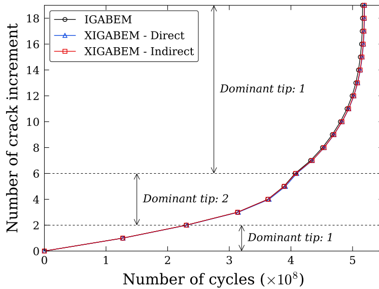
Figure 35: Incremental fatigue process for the perforated panel determined by the unenriched and enriched formulations.
