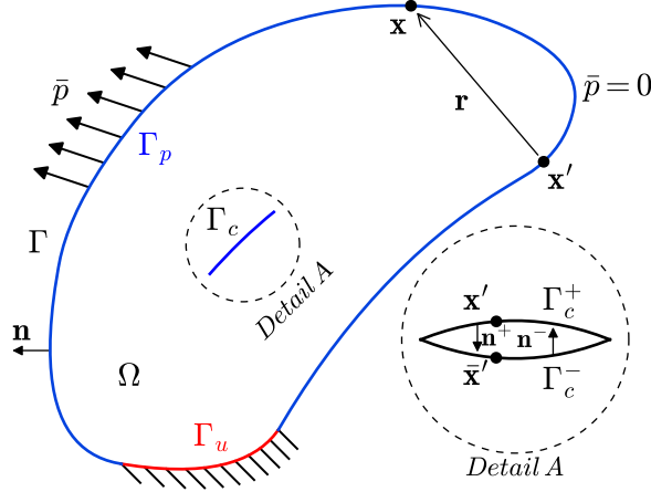
Figure 3: Representation of a cracked body.
