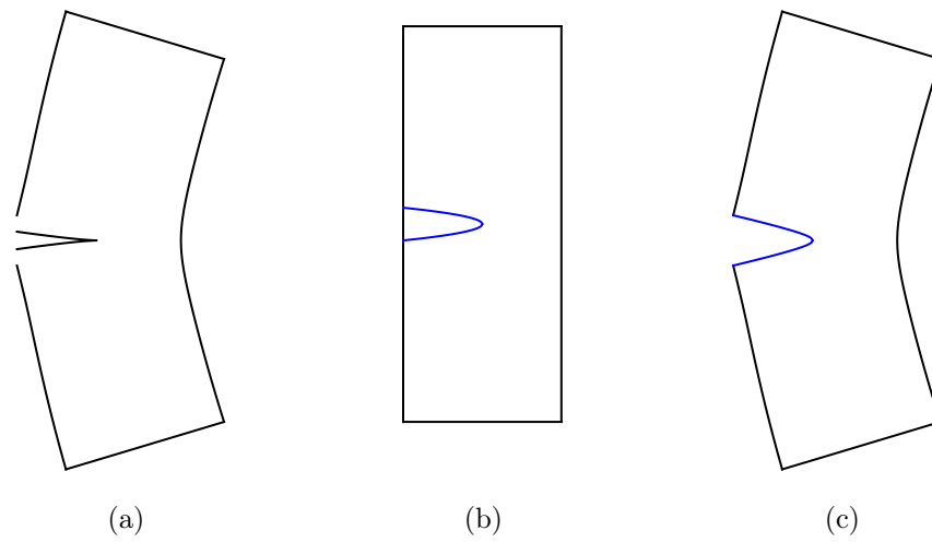
Figure 15: Deformed shapes considering the contribution from (a) the NURBS basis functions and (b) the enrichment term. (c) Final deformed shape for pure mode I problem, given by the superposition of solutions from (a) and (b). The enriched NURBS are depicted in blue (please refer to the coloured version).
