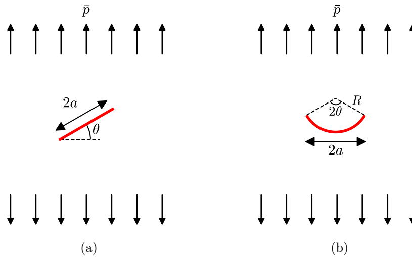
Figure 16: Cracks in an infinite domain submitted to far-field vertical loading: (a) Inclined crack and (b) circular arc crack.
