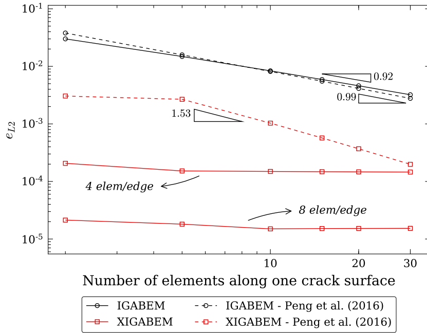
Figure 10: Relative L^2 displacement error norm e_{L2} (Eq. (32)) along the crack surfaces. The reference results are taken from Peng et al. [42].
