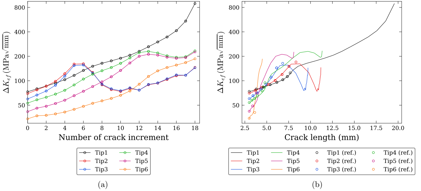
Figure 33: Variation of \Delta K_{ef} with (a) crack increment and (b) crack length.
