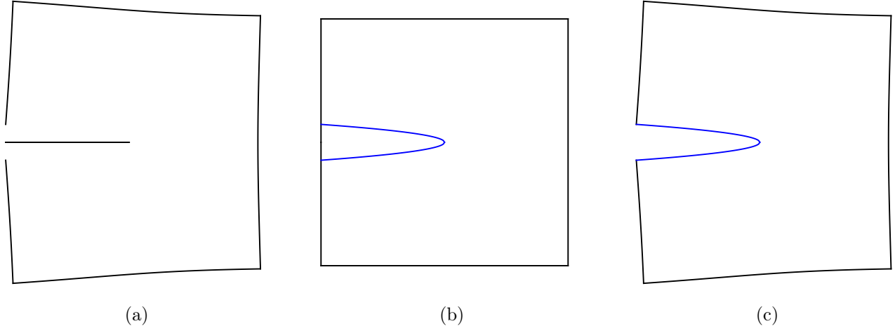
Figure 11: Deformed shapes considering the contribution from (a) the NURBS basis functions and (b) the enrichment term. (c) Final deformed shape for pure mode I problem, given by the superposition of solutions from (a) and (b). The enriched NURBS are depicted in blue (please refer to the coloured version).
