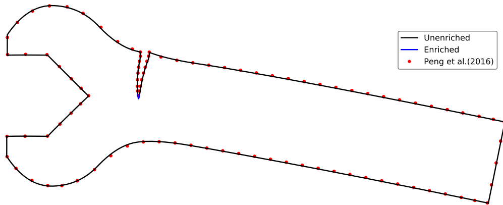
Figure 26: Deformed shape after ten crack increments obtained with the XIGABEM model considering the direct method for SIF extraction. The segments near the crack tip containing the enrichment term for the displacement approximation are depicted in blue (please refer to the coloured version). The solution provided by Peng et al. [42] is also shown for comparison.
