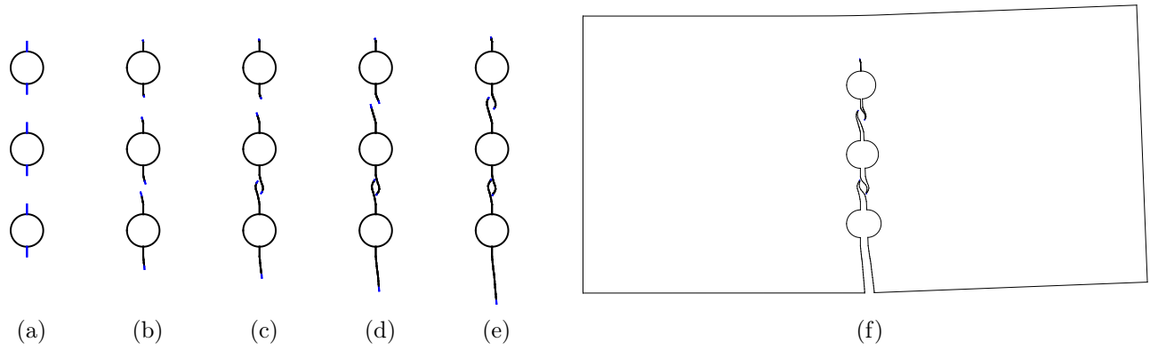
Figure 34: (a)-(e) Evolution of the crack paths and (f) final deformed shape obtained by the direct XIGABEM formulation. The enriched NURBS segments are depicted in blue (please refer to the coloured version).
