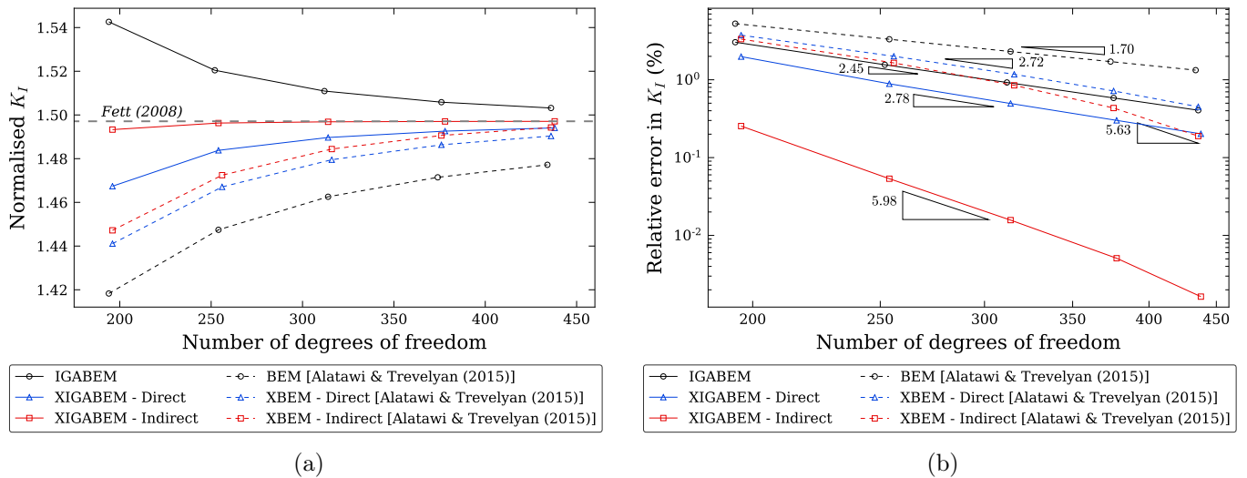
Figure 14: Variation of (a) mode I SIF (normalised by \bar{\sigma}\sqrt{\pi a} ) and (b) relative error with the mesh refinement obtained by the present work and by Alatawi and Trevelyan [46]. The reference value for normalised K_I is taken from Fett [68].
