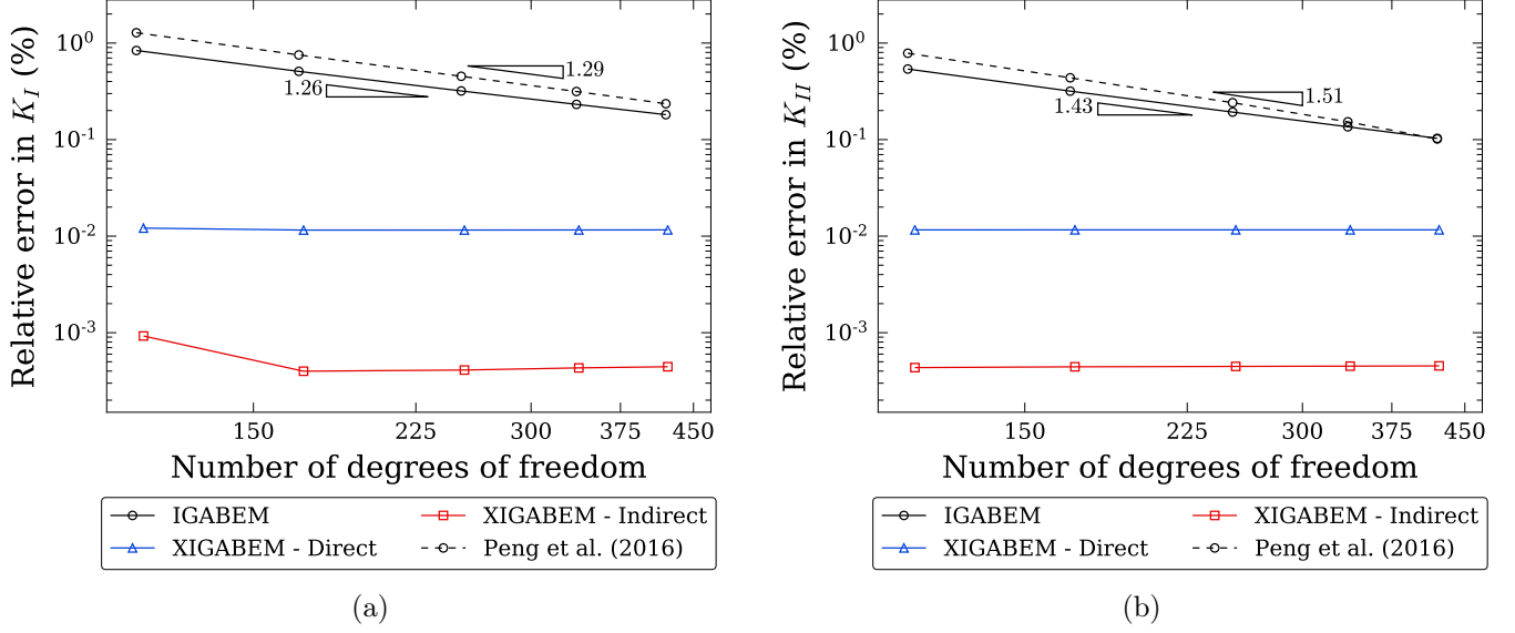
Figure 12: Convergence of (a) mode I and (b) mode II SIF.
