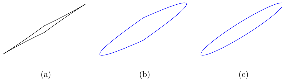
Figure 19: Deformed shapes for inclined crack ( \theta = 30^\circ ) considering the contribution from (a) the NURBS basis functions and (b) the enrichment term. (c) Final deformed shape for inclined crack, given by the superposition of solutions from (a) and (b). Enriched NURBS are depicted in blue (please refer to the coloured version).
