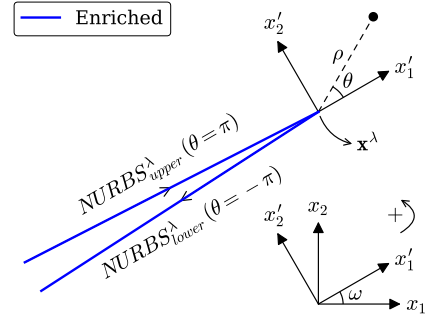
Figure 5: Local coordinate system at an enriched crack tip.
