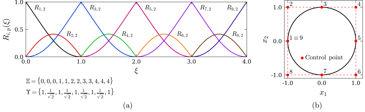
Figure 1: Representation of (a) the NURBS basis functions and (b) the NURBS curve representing a unit circle. The order of the NURBS is p = 2 .
