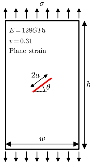
Figure 22: Rectangular specimen of a titanium plate with a central inclined crack.
