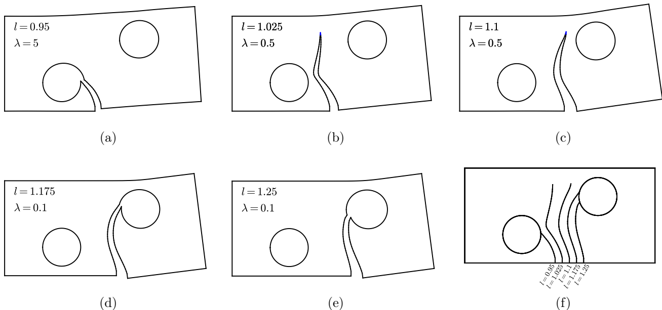
Figure 29: Deformed shape for the configuration considering (a) l = 0.95 , (b) l = 1.025 , (c) l = 1.1 , (d) l = 1.175 and (e) l = 1.25 . The scale factor \lambda used in each figure is also indicated. The NURBS segments near the crack tip containing the enrichment term for the displacement approximation are depicted in blue (please refer to the coloured version). Note that in the models where the crack crosses a boundary, the enrichment is removed from the near-tip elements since the analytical square root behaviour no longer exists once the intersection occurs. (f) Crack paths determined for each initial crack position.
