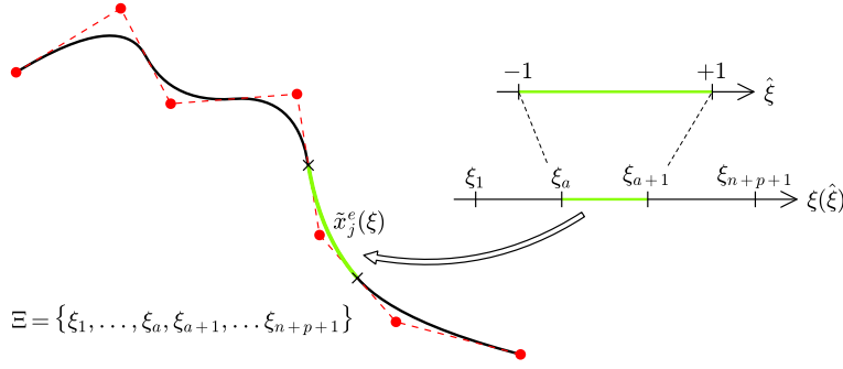
Figure 4: Mapping between the Cartesian, parametric and the parent spaces.
