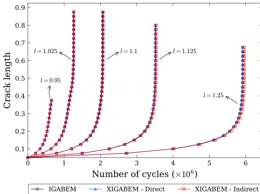
Figure 30: Crack length evolution determined by the unenriched and enriched formulations considering the different values of l .
