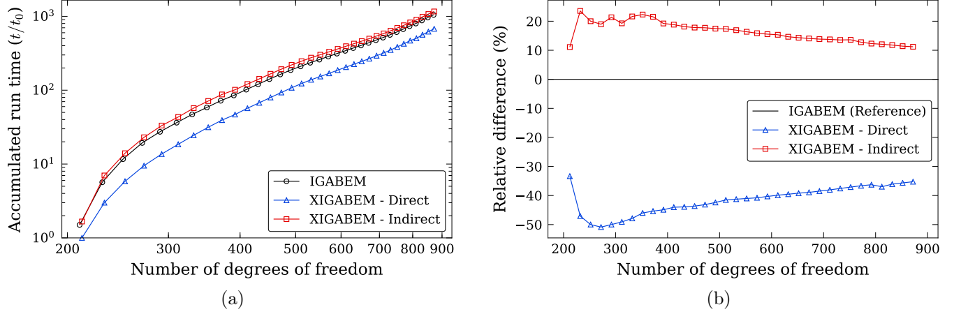
Figure 31: (a) Accumulated run time to obtain the solution for each crack configuration. The values are normalised by t_0 = 93.7 ms, which is the smallest time observed among the analyses of the initial configuration and corresponds to that obtained in the direct XIGABEM. (b) Relative differences between accumulated run times considering the indirect IGABEM results as reference.
