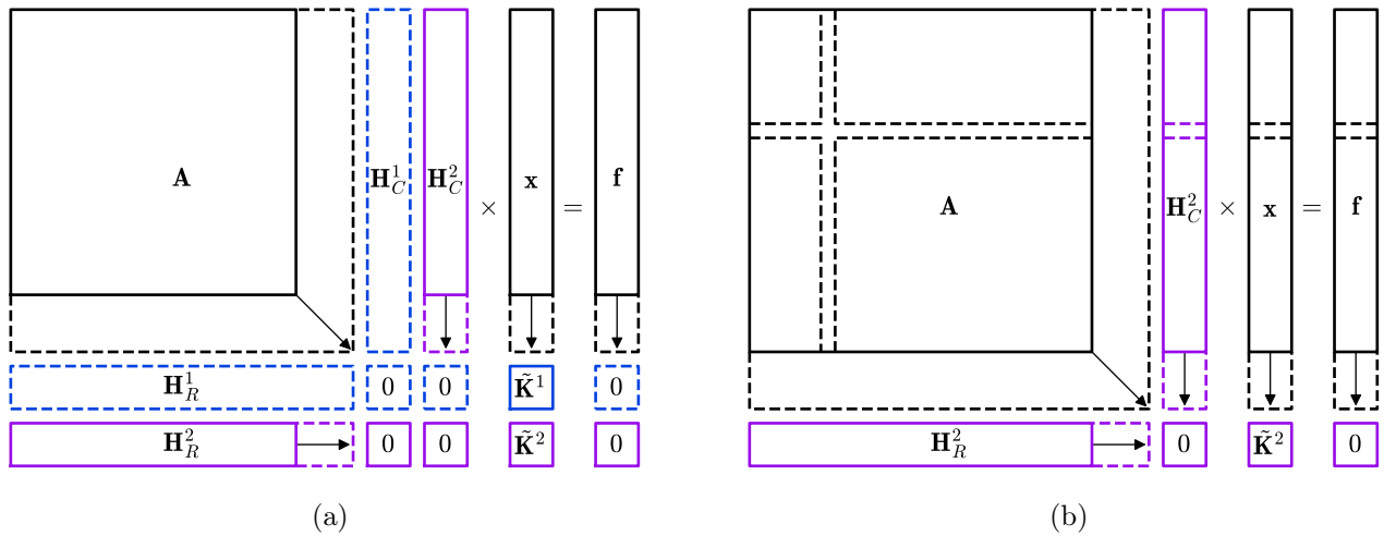
Figure 7: Graphical representation of the changes in the sub-matrices from the system of equations resulting from (a) the crack propagation illustrated in Fig. 6b and (b) the crack propagation followed by the intersection of a NURBS depicted in Fig. 6c. Note that most of the sub-matrices remain unaltered (represented by solid lines). The changes in the system (represented by dashed lines) are related to the enrichment parameters related to the growing tip and the new control/collocation points defined along the new crack surfaces and intersected NURBS.
