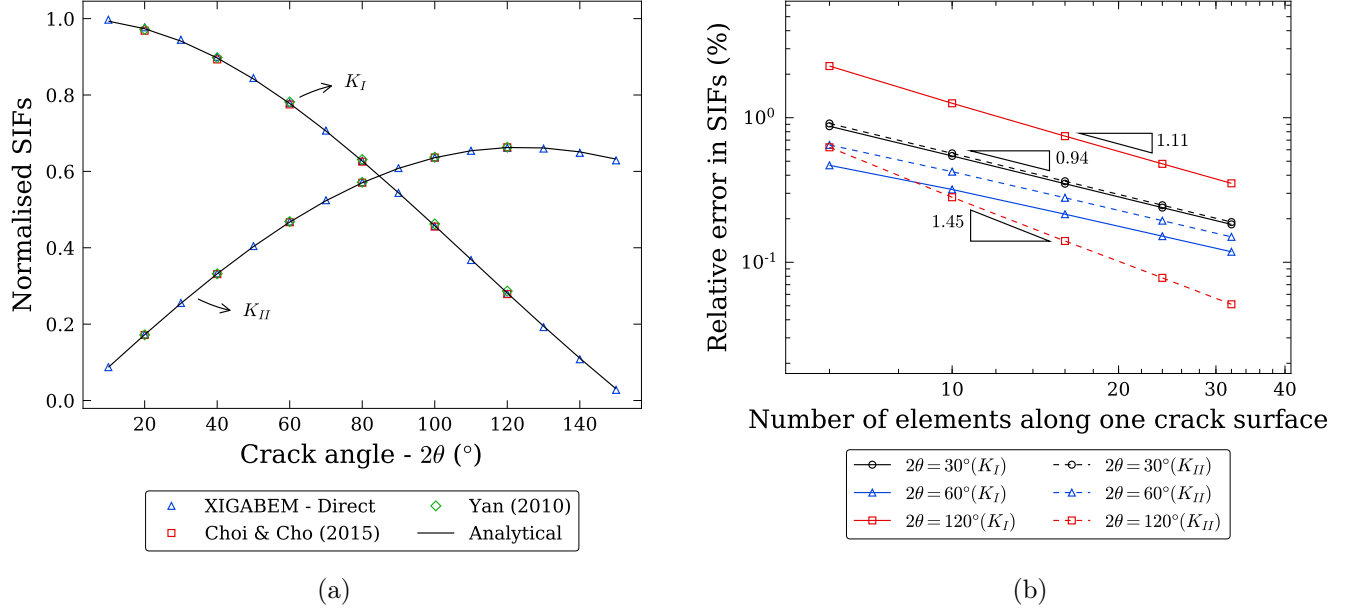
Figure 20: (a) Results for normalised SIFs for circular arc crack considering 16 elements in each crack surface. (b) Relative error evolution with crack mesh refinement.
