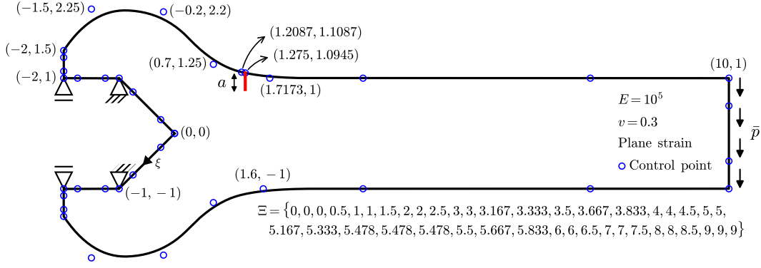
Figure 25: Open spanner with an edge crack. The repeated knot 5.478 in the knot vector defining the external boundary indicates the position of the crack mouth. Besides, the weights associated with the control points are taken as a unit.
