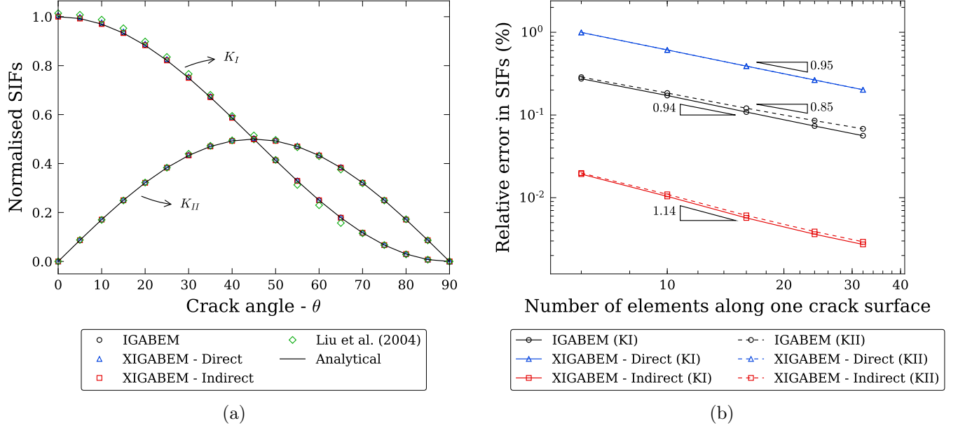
Figure 17: (a) Results for normalised SIFs for inclined crack considering 10 elements in each crack surface. (b) Relative error evolution with crack mesh refinement.
