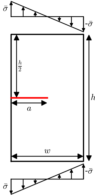
Figure 13: Rectangular plate with an edge crack under uniform loading.
