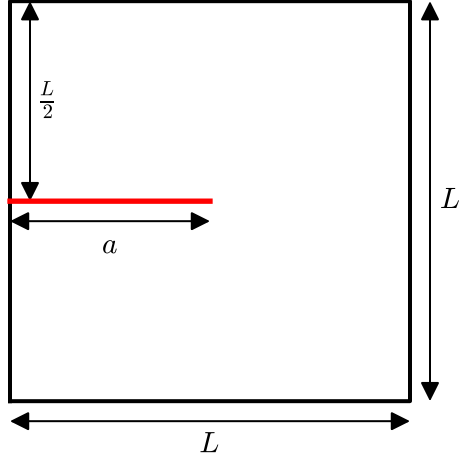
Figure 8: Square plate with an edge crack.
