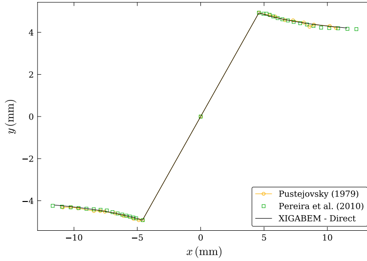
Figure 23: Comparison between the propagation path obtained by the XIGABEM model considering the direct approach for SIFs extraction and the experimental results determined by Pustejovsky [75]. The numerical solution obtained by Pereira et al. [76] using GFEM is also provided.
