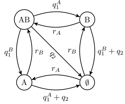
Figure 1: Markov chain for failure with non-instant repair. The nodes show non-faulty power lines.
