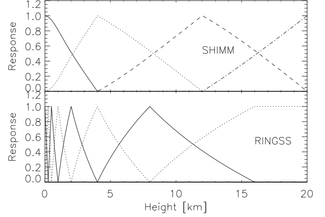
Figure 8. A plot of the response functions for the 24hSHIMM and RINGSS. The alternating line styles differentiate the response functions of each reconstructed layer. The sum of responses from all layers is approximately one.
