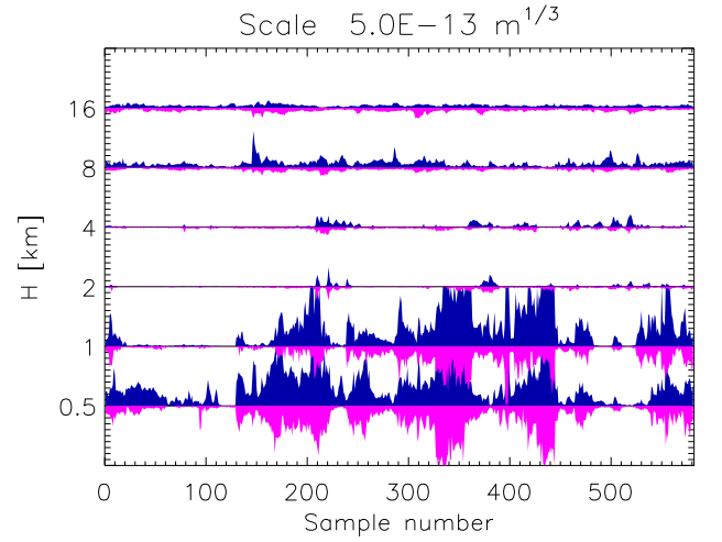
Figure 10. Turbulence profiles measured simultaneously by RINGSS (up-facing blue bars) and S-SCIDAR (down-facing magenta bars). S-SCIDAR is matched in resolution and time to RINGSS with the sample number indicating the n th S-SCIDAR measurement taken during the campaign. The width of each band is 5 \times 10^{-13} \text{ m}^{1/3} .
