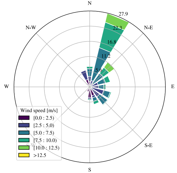
Figure 6. A wind rose displaying the distribution of wind speeds and directions measured 30 m above the ground by the Paranal meteo-tower for the six nights of the campaign.
