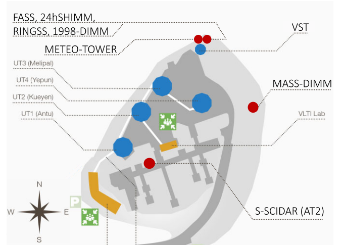
Figure 1. Location of turbulence monitoring instrumentation described in Section 2. Instruments relevant to this study are indicated by the smaller circles and bold labels. Original image credit: ESO.
