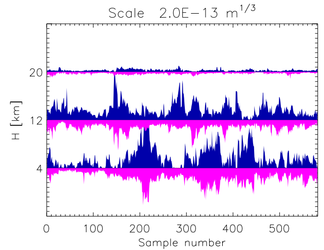
Figure 11. Turbulence profiles measured simultaneously by 24hSHIMM (up-facing blue bars) and S-SCIDAR (down-facing magenta bars). S-SCIDAR is matched in resolution and time to 24hSHIMM with the sample number indicating the n th S-SCIDAR measurement taken during the campaign. The width of each band is 2 \times 10^{-13} \text{ m}^{1/3} .
