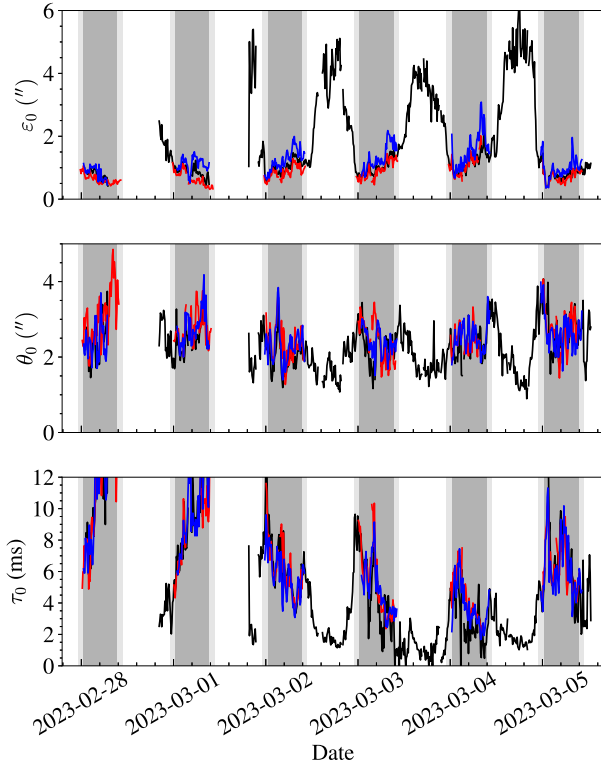
Figure 12. Integrated parameters measured by the 24hSHIMM during the campaign. The black line represents 24hSHIMM measurements, the red line DIMM measurements for seeing and MASS-DIMM for the coherence time and isoplanatic angle, and the blue line the RINGSS. All data sets have been binned to 10-min intervals for presentation and dates are in UTC. The white, grey, and light grey shades of the background represent daytime, night, and twilight, respectively.
