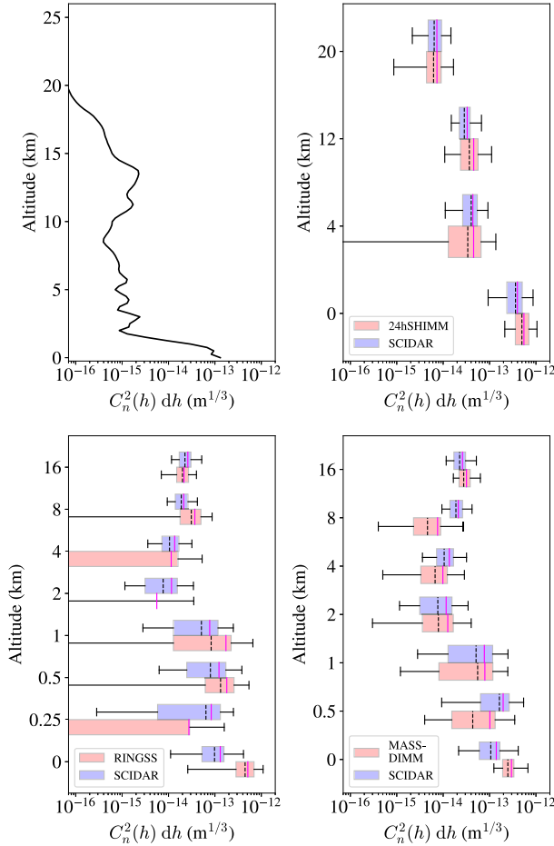
Figure 9. A comparison of C_n^2(h) dh profile measurements for all instruments with contemporaneous measurements from the S-SCIDAR. The red boxes offset below the altitude markers show the instrument data from each fitted layer, and the blue boxes above the altitude markers the contemporaneous measurements (within \pm 2 min) from the S-SCIDAR which have been binned to match the instrument layers using the response functions. The extent of coloured boxes represents the first and third quartiles, the dashed line the median measurement, the magenta line the mean, and the whiskers the fifth and 95th percentiles of the distribution. From top left to bottom right, the plot shows the mean S-SCIDAR profile, and box and whisker plots for the 24hSHIMM, RINGSS, and MASS-DIMM compared with S-SCIDAR. Significantly smaller values in the top-left panel, compared to other panels, are explained by the thinner dh = 0.25 km layers of the S-SCIDAR profiles.
