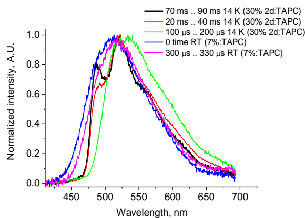
Figure S1 Late time delayed emission from 2d :TAPC film at 14 K and RT.
