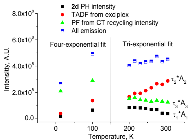
Figure S4. Integrated intensities of DF, PF and PH (as described in Figure S1) and total emission. DF intensity increases with temperature whereas PH and PF intensities decrease. This results in an overall intensity increase >200 K. The intensities were calculated using fitting results from Table S1.
