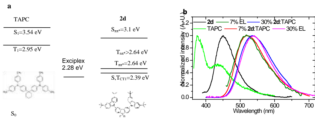
Figure 2. a) Structures and singlet, triplet levels of investigated molecules in the emitter layer. Triplet singlet levels of excitonic state have been taken as onsets from spectra from our measurements of 2d :TAPC film for 2d and literature for TAPC. [24, 25] CT and exciplex energies are the average energy of the transition taken from the spectral peak position. b) Steady state PL spectra of 2d and TAPC neat films and 2d in TAPC at 7% and 30% loading. TAPC film PL: \lambda_{\max} 371 nm and TAPC excimer/dimer: \lambda_{\max} 468 nm.
