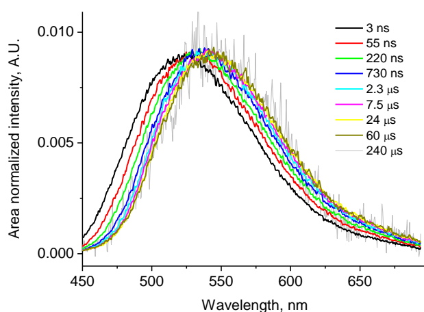
Figure S6. Time resolved area normalized spectra of 40% 2d doped in TAPC. Isoemissive point is not visible.
