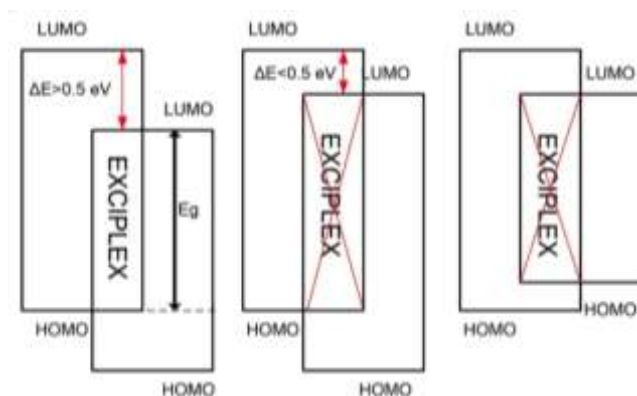
Figure S7. Exciplexes are formed between 2d and a material which has at least \sim 0.5 \text{ eV} higher LUMO and higher HOMO as shown in Figure 5.
