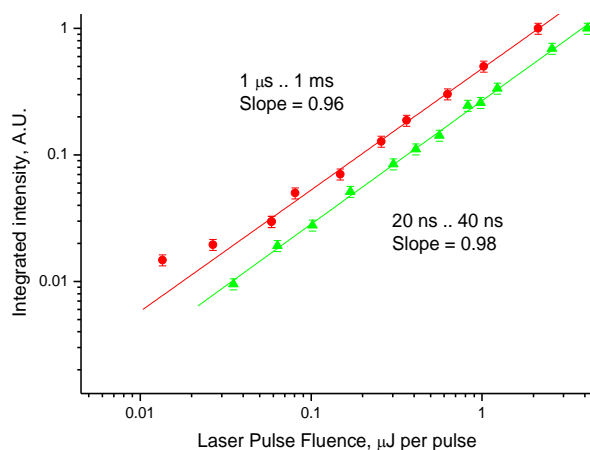
Figure S2. 30% 2d :TAPC Emission intensity dependence on excitation laser fluence. Triangles and circles are experimental points at indicated delay and gate times, straight lines are fits in log-log scale.
