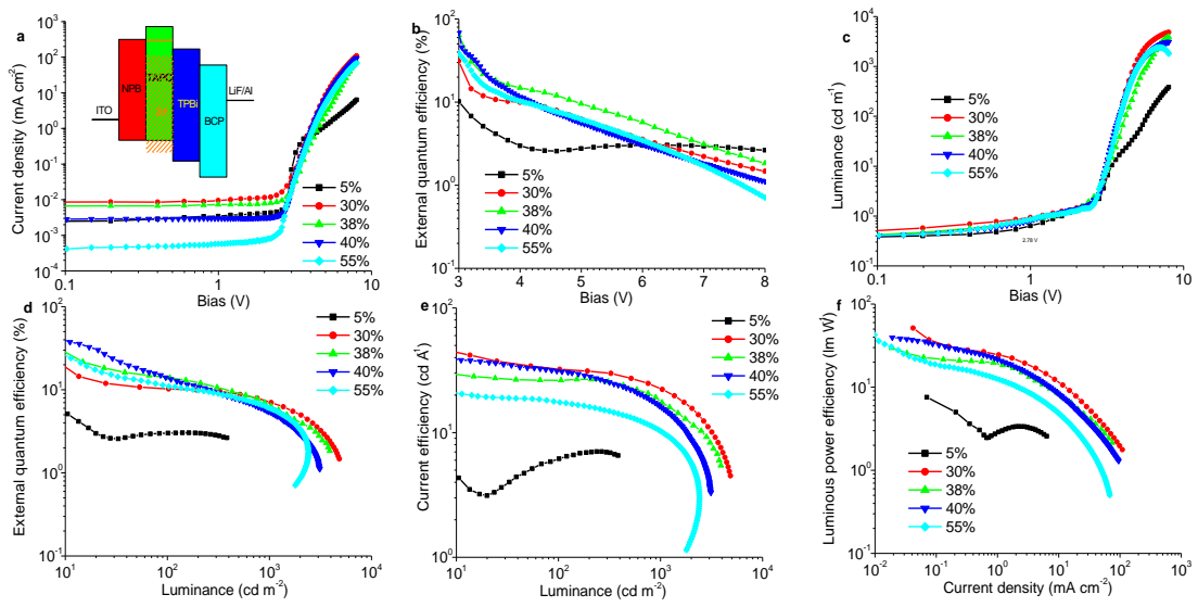
Figure 1. 2d:TAPC OLED characteristics. a) Current density vs bias, b) EQE vs bias, c) luminance vs bias, d) EQE vs luminance, inset, characteristics of devices at 100 cd/m 2 and 1000 cd/m 2 brightness, e) current efficiency vs luminance, f) power efficiency vs current density. The abnormally high EQE at very low brightness may be an artefact of making the measurement in a large 10 inch integrating sphere. Percentages of 2d dopant, by weight, are indicated.
