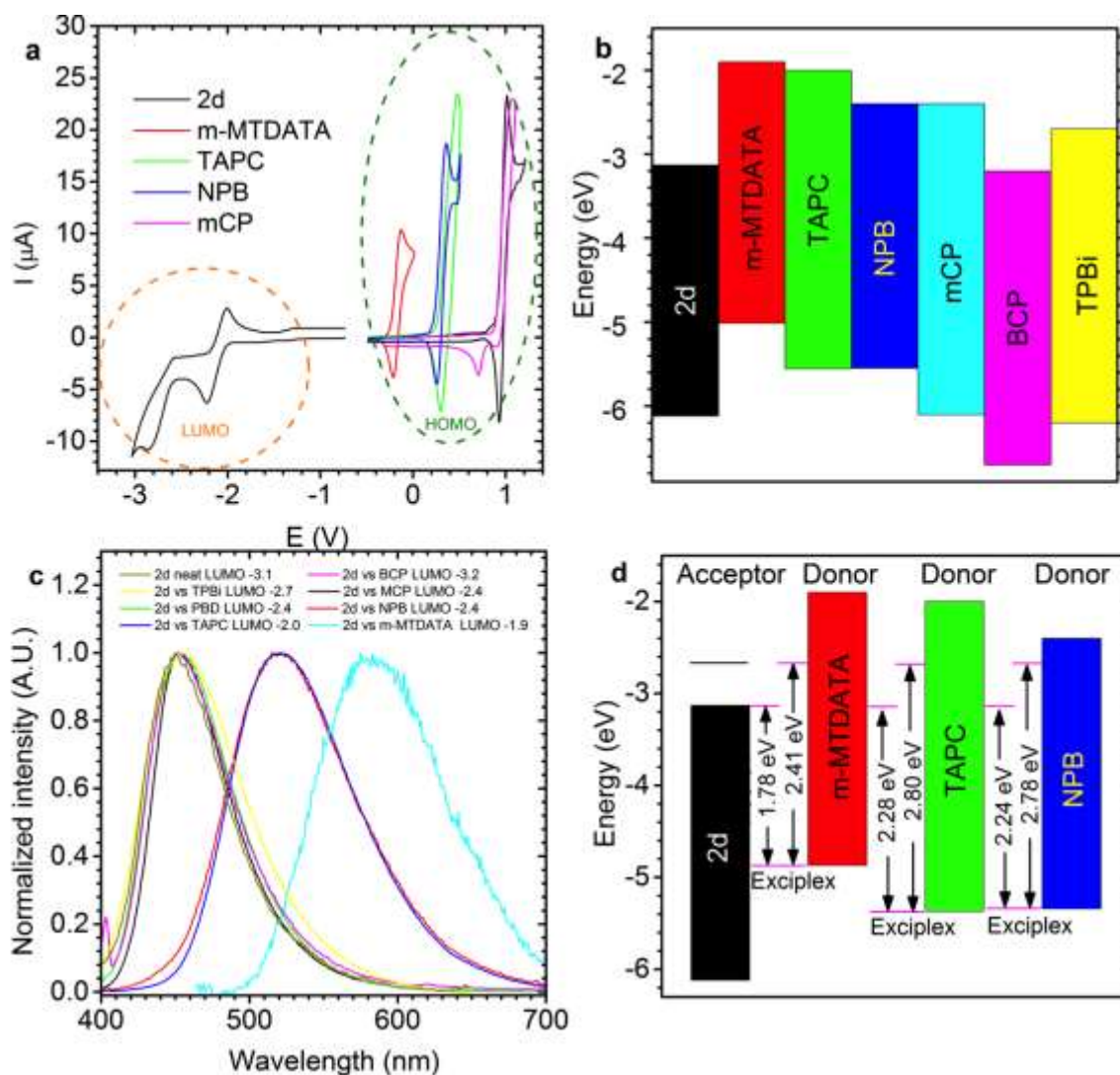
Figure 5. a , CV characteristics of 2d and a small range of donor molecules; b , The HOMO-LUMO levels determined from the redox levels of the molecules; c , Emission spectra of 2d and 50:50 mixtures of 2d and the various donor molecules which clearly shows a differentiation between donors which can and those that cannot form an exciplex with 2d ; different hosts; d , HOMO don -LUMO acc levels and energy differences of the formed exciplexes.
