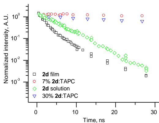
Figure S3. Decays of 7% 2d :TAPC, 30% 2d :TAPC and neat film recorded at 10 \mu\text{J} per pulse at RT in log-lin scale. Decay of 2d in solution is included for comparison.
