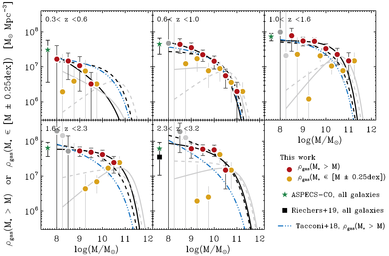
Figure 11. Same as Figure 7 but here the gas mass densities are inferred using a gas-to-dust mass ratio–metallicity relation with a much steeper power-law at metallicity < 7.9 ( \sim 3 ; Rémy-Ruyer et al. 2014).
