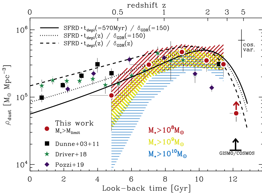
Figure 6. Evolution with look-back time (lower x -axis; or redshift, upper x -axis) of the comoving dust mass density in galaxies derived here using the ASPECS LP 1.2 mm continuum map. Red circles are for galaxies with M_* > M_{\text{limit}} , as inferred from Figure 4. Red, yellow, and blue hashed regions are inferred from the best-fits of \rho_{\text{dust}}(M_* > M, z) (see Figure 4) and correspond to the cosmic dust mass densities in galaxies with M_* > 10^8 M_\odot , M_* > 10^9 M_\odot , and M_* > 10^{10} M_\odot , respectively. These best-fits were performed independently for each redshift bin. At z > 3 , we derive lower limits by stacking all galaxies in our H -band-selected sample, irrespective of their stellar masses. At a similar redshift, we show the lower limit inferred by Magnelli et al. (2019) using a 2 mm selected galaxy sample. Black squares, green stars, and dark blue diamonds show the total comoving dust mass densities in galaxies inferred by Dunne et al. (2003, 2011), Driver et al. (2018), and Pozzi et al. (2019), respectively. The solid line shows predictions from scaling the cosmic SFRD (Madau & Dickinson 2014) assuming a redshift-independent gas depletion timescale ( t_{\text{depl}} = M_{\text{gas}}/\text{SFR} ) of 570 Myr and a gas-to-dust mass ratio of 150; both values being typical for 10^{10.3} M_\odot main-sequence star-forming galaxies at z \sim 2 (Tacconi et al. 2018). The dotted line shows predictions assuming a gas-to-dust mass ratio of 150 but a redshift-dependent gas depletion time as parametrized by Tacconi et al. (2018) for 10^{10.3} M_\odot main-sequence star-forming galaxies (i.e., t_{\text{depl}} = 570 Myr at z = 2 and 860 Myr at z = 0 ). Finally, the dashed line shows predictions assuming both a redshift-dependent depletion time and gas-to-dust mass ratio. This latter is derived from Equation (2) using the metallicity of 10^{10.3} M_\odot galaxies at a given redshift (Equation (3)). This yields \delta_{\text{GDR}} = 150 at z = 2 and \delta_{\text{GDR}} = 90 at z = 0 . The typical fractional cosmic variance uncertainty of \sim 45\% affecting our measurements and inferred using the methodology advocated by Driver & Robotham (2010) is illustrated in the upper right-hand corner.
