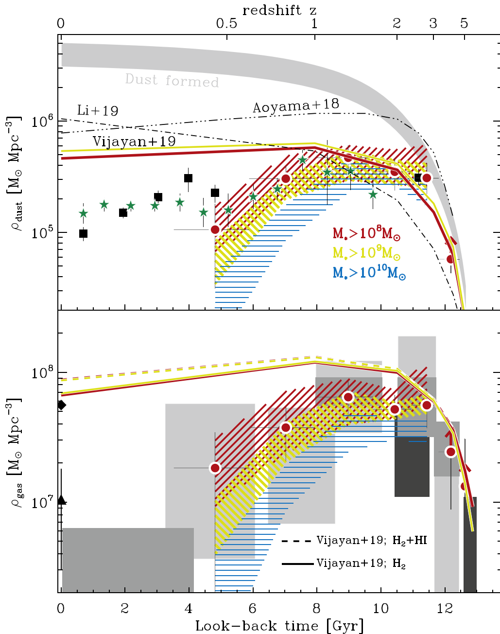
Figure 13. Same as Figure 10 but here we compare our measurements to predictions from the semi-analytical model of Vijayan et al. (2019). For M_* > 10^9 M_{\odot} , we used their “Millennium” predictions, while for M_* > 10^8 M_{\odot} we use their “Millennium-II” predictions.
