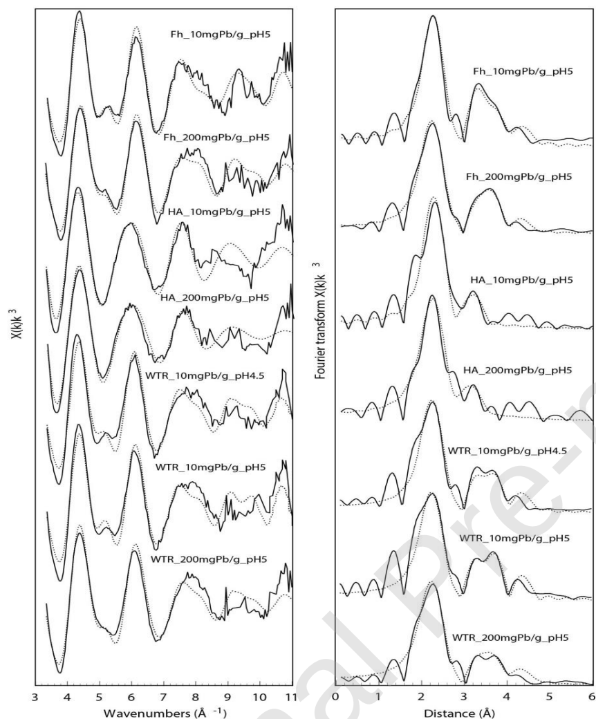
Figure 7. Lead L_{III} -edge EXAFS spectra for Pb(II) adsorbed on WTR, ferrihydrite (Fh) and humic acid (HA). (A) k^3\chi(k) functions; (B) corresponding RSFs (uncorrected phase shift). The experimental data (solid line) are fitted (dashed line) using the parameters described in the text.
