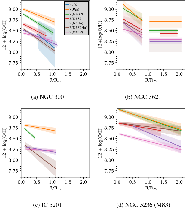
Figure 10. The set of measured metallicity gradients for each host galaxy determined in the integrated-region study, as listed in Tables 6 and 7. Gradients are distinguished by metallicity method as indicated by the legend shown in panel 10(a), with 1\sigma uncertainty bands also shown around each line. Detailed versions of these plots as well as literature comparisons are shown in Figs A2 to A5.
