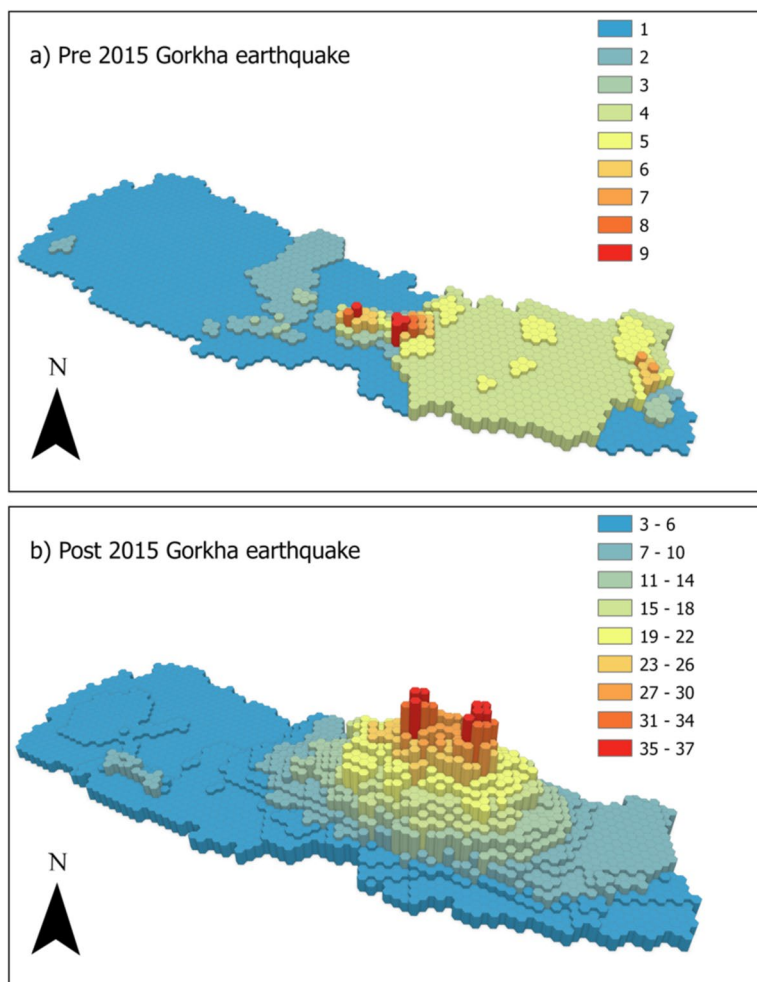
Fig. 4 Number of landslide inventories per 10 km 2 hexagonal tile. (a) The spatial pattern and numbers of landslide inventories produced using data collected prior to the 2015 Gorkha earthquakes. Note concentrations near Kathmandu in central Nepal and the Koshi Basin in eastern Nepal. (b) As panel a, but using data collected following the Gorkha earthquakes. Thirteen studies did not provide an indication of when the landslide inventory was created and therefore have been excluded from the count. If a landslide inventory was published before 2015 but did not give a date range, we included the inventory in panel (a). Where landslide inventories were multi-temporal, we considered the date of the final inventory and therefore most multi-temporal inventories are included in panel (b), as they tended to focus on the change in landsliding before and after the 2015 earthquakes. North is toward the top of both panels
