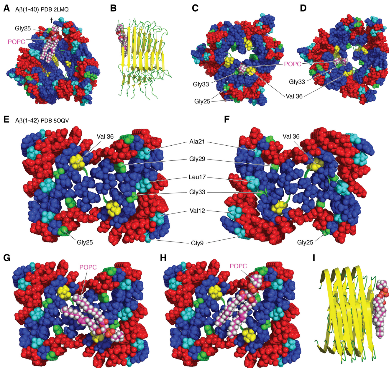
Figure 5. Representations of potential lipid-binding sites in fibrils of Aβ. In each case, a molecule of POPC has been manually docked onto a known peptide structure in an orientation and position consistent with proximity data from solid-state NMR measurements in order to illustrate relative size and fit. Hydrophobic and hydrophilic residues are colored blue and red , respectively (with His assigned as hydrophilic and Tyr as hydrophobic), apart from specific residues that are labeled in each structure. A and B , show an end view ( space filling ) and side view ( cartoon ) of an Aβ(1–40) structure with spherical symmetry (PDB ID: 2LMQ (135)) with a POPC molecule intercalated in the β-sheet structure. The side chain of Tyr10 is indicated with a dagger . C and D , show the same structure as A/B , but with a POPC molecule incorporated in the central cavity. Residues 1 to 8 of Aβ(1–40) are missing from this structure. However, residue 9 lies on the outside of the structure away from the central cavity. E and F , show opposing faces of an Aβ(1–42) fibril composed of two proto-filaments (PDB ID: 5OQV (142)) with helical symmetry, looking along the axis of the fibril. G and H , show POPC molecules docked onto the structure in E . I , shows a cartoon representation of the side view of the structure in H . Aβ(1–40), fragment 1 to 40 of the amyloid-β peptide; PDB, Protein Data Bank; POPC, 1-palmitoyl-2-oleoyl- sn -glycero-3-phosphocholine.
