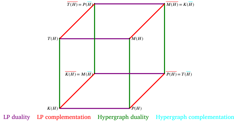
Fig. 2. The eight Linear Programs related to a hypergraph.
