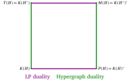
Fig. 1. The four initial Linear Programs related to a hypergraph. (For interpretation of the colours in the figure(s), the reader is referred to the web version of this article.)
