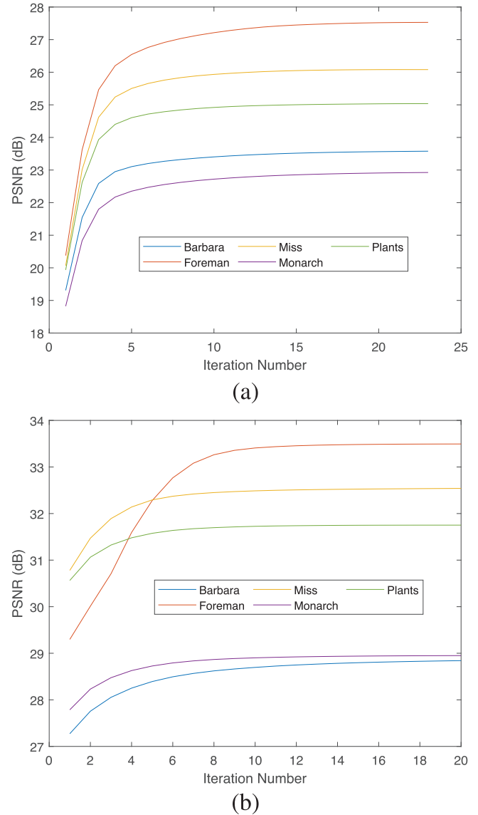
FIGURE 12 Convergence of the proposed algorithm with various strategies: (a) how PSNR changes as the number of iterations increases with noise level \sigma_E = 50 and (b) how PSNR changes as the number of iterations increases with compression quality Q = 10 .
