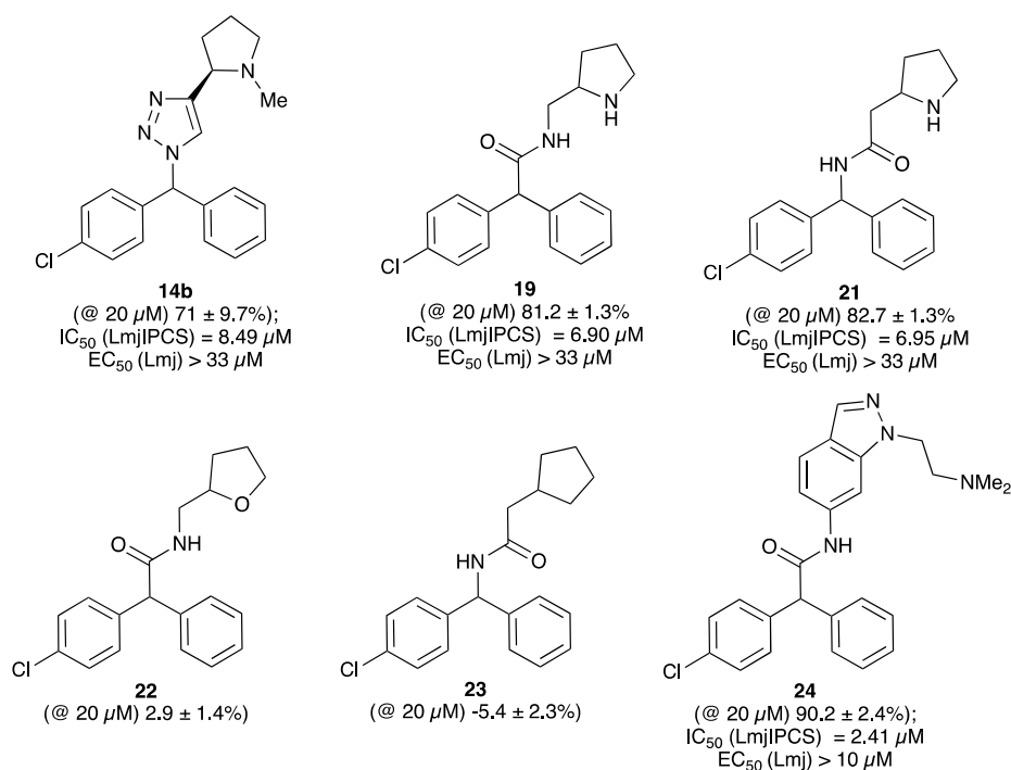
Figure 2: Activity of a selection of simple amide and triazole linked CF analogues against a microsomal preparation of L.maj IPCS and L.major promastigote parasites, respectively. Values in parenthesis indicate relative inhibition of the enzyme preparation at 20 μM. For further details and a full list of analogues see SI.
