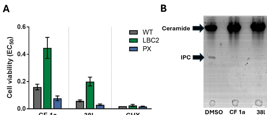
Figure 3: On-target Assays for Analogue 38I. A EC 50 values of CF 1a and analogue 38I against WT, \Delta LCB2 and PX L. major promastigotes; CHX, cycloheximide, was used as a positive control; values are presented as mean \pm 95% CI from at least three experiments. B Separation of NBD- C_6 -IPC 81 product from NBD- C_6 -ceramide 80 substrate by HPTLC; Microsomes were treated with 5mM of analogue 38I and negative and positive controls were DMSO and 5mM of CF 1a , respectively.
