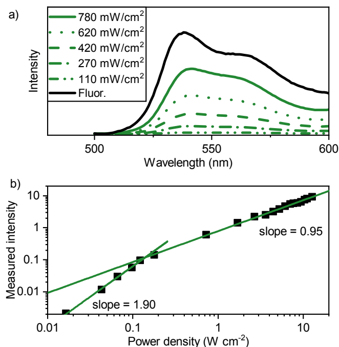
Figure 4: a) Emission spectra of a PdTNP-tetracene film (evaporated; 500 nm on quartz, 1% PdTNP, green lines) with incident power of the laser beam indicated ( I_{\text{exc}} = 690 nm, CW, \phi = 2 mm). In black the conventional fluorescence spectrum ( I_{\text{exc}} = 475 nm) of a neat tetracene film is shown, b) Power density dependence of the PdTNP-tetracene thin film emission, excited at 690 nm.
