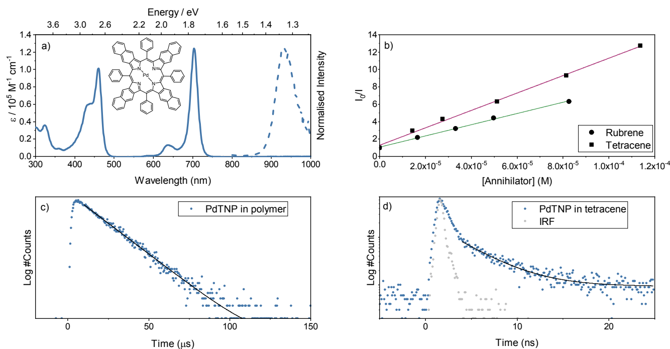
Figure 3: a) Absorbance (solid) and emission (dashed, I_{\text{exc}} = 705 nm) spectra collected for the porphyrin, PdTNP (5 mM in toluene). b) Stern-Volmer plot for the dynamic quenching of PdTNP by both mediator and annihilator ( I_{\text{em}} = 930 nm, toluene). c) Phosphorescence decay of 1% PdTNP in polystyrene (processed by spin coating) using the multichannel scaling technique ( I_{\text{exc}} = 705 nm). d) Phosphorescence decay of 1% PdTNP in tetracene using the TCSPC technique ( I_{\text{exc}} = 475 nm, I_{\text{em}} = 930 nm, 500 nm on quartz, blue dots), grey dots indicate the measured IRF.
