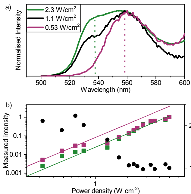
Figure 5: a) Normalized emission spectra of PdTNP-tetracene-rubrene films (evaporated; 500 nm on quartz, 1% PdTNP and 1% rubrene) with incident power of the laser beam indicated ( \lambda = 690 nm, CW, \phi = 2 mm). The vertical dashed lines indicate the fluorescence maximum of neat films of tetracene (green) and rubrene (purple), indicating the likely emitter species. b) Power density dependence of the ternary blended thin film emission measured at 540 nm (green squares) and 560 nm (purple squares) using 4 nm slight widths, together with the ratio between the two signals (black circles).
