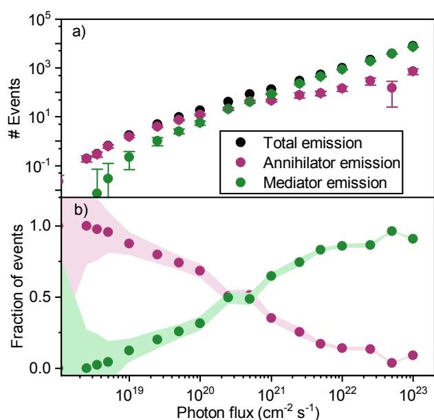
Figure 7: a) Simulated emission events resulting in emission in a ternary blend with 1% sensitizers and 0.1% of annihilators in a host (mol/mol). b) Simulated fraction of upconversion events due to hetero-TTA (purple) and homo-TTA (green).
