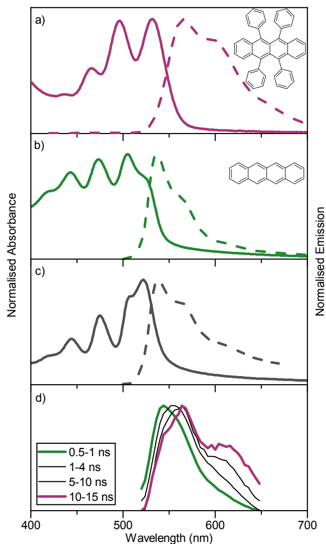
Figure 2: Absorption and steady-state emission spectra for evaporated films of a) rubrene, b) tetracene, and c) 5% rubrene in tetracene ( I_{exc} = 475 nm), taken as 100 nm
