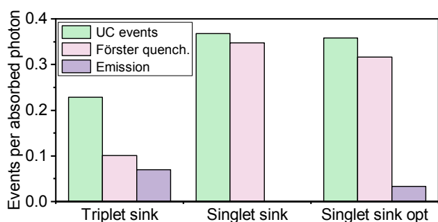
Figure 8: Comparison of the singlet sink approach and the proposed mediator-based approach (Triplet sink). All parameters in the simulations are the same for the two systems except that for the mediator approach the rate of homo-TTA was set to 0, and for the singlet sink approach the rate of hetero-TTA was set to 0. The concentration of annihilators was increased from 10^{-3} to 10^{-2} for the optimized singlet sink approach (Singlet sink opt). Simulations were performed using a photon flux of 10^{20} photons \text{cm}^{-2} \text{s}^{-1} .
