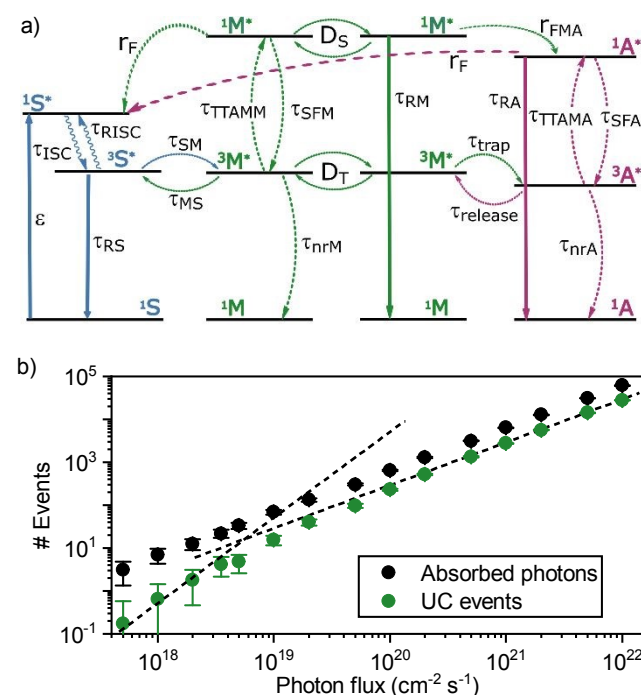
Figure 6: a) Scheme of the rates used in the Monte-Carlo simulations. The values of rates are given in Table S1. b) Emission events as a function of the incident photon flux for a system of 1% sensitizers in a host matrix (tetracene). The two dashed lines have a slope of 1 and 2 as visual guides.
