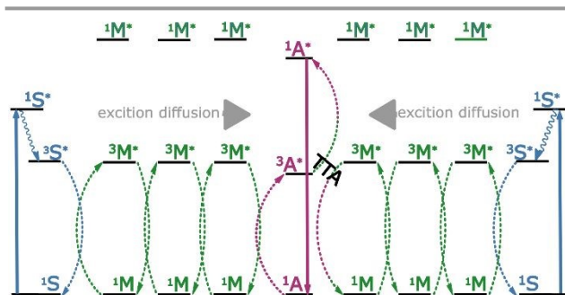
Figure 1: Schematic diagram of the energy transfer pathways and the photon upconversion mechanism in this work. Photon absorption and ISC occurs on the sensitizer (S), and triplet energy transfer to the mediator (M) proceeds with high efficiency. Exciton diffusion between mediators is rapid and occurs over long distances, resulting in hetero-TTA at the annihilator(A) sites.
