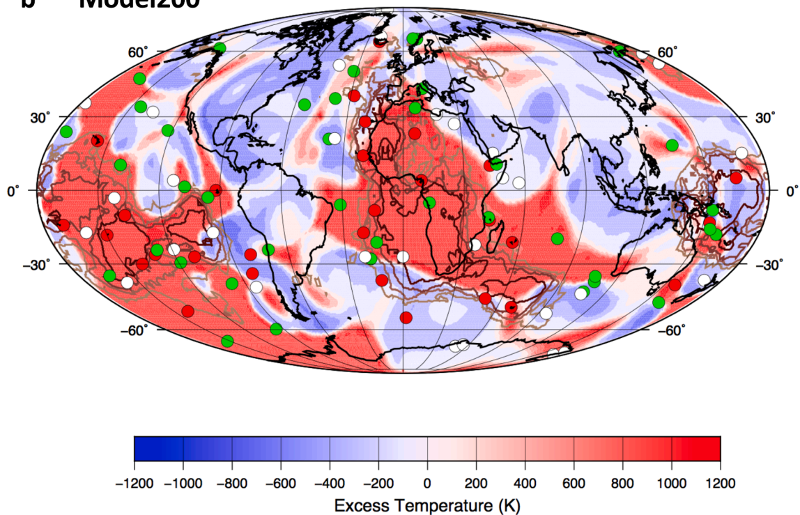
Fig. 14. Comparison between Model200 and Model200hr (a higher resolution simulation). The excess temperature at 2800 km depth for Model200hr is given in (a), with seismic tomography velocity contours as Fig. 1. Green circles and white circles show Model200 and Model200hr plume positions, respectively. Red circles are of the approximate present-day plume database (Table 3). See Methods for Model200hr description. The excess temperature at 2800 km depth for Model200 is given in (b) for comparison. Circles as (a). (For interpretation of the references to colour in this figure legend, the reader is referred to the web version of this article.)
