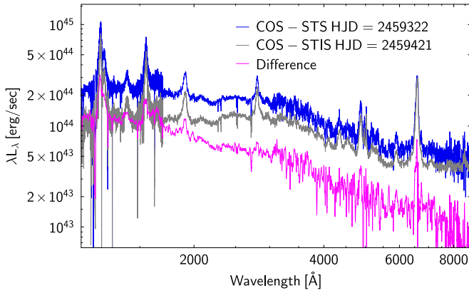
Figure 2. A comparison of two COS-STIS spectra obtained during periods of high ( v75 , HJD = 2459322) and low ( v30 , HJD = 2459421) 1144 Å flux levels. The magenta curve shows the difference between the two spectra. The similarity of the spectra at long wavelengths compared with a factor of \approx 2 difference in the 1144 Å flux suggests a significant change in the shape of the SED between the two epochs.
