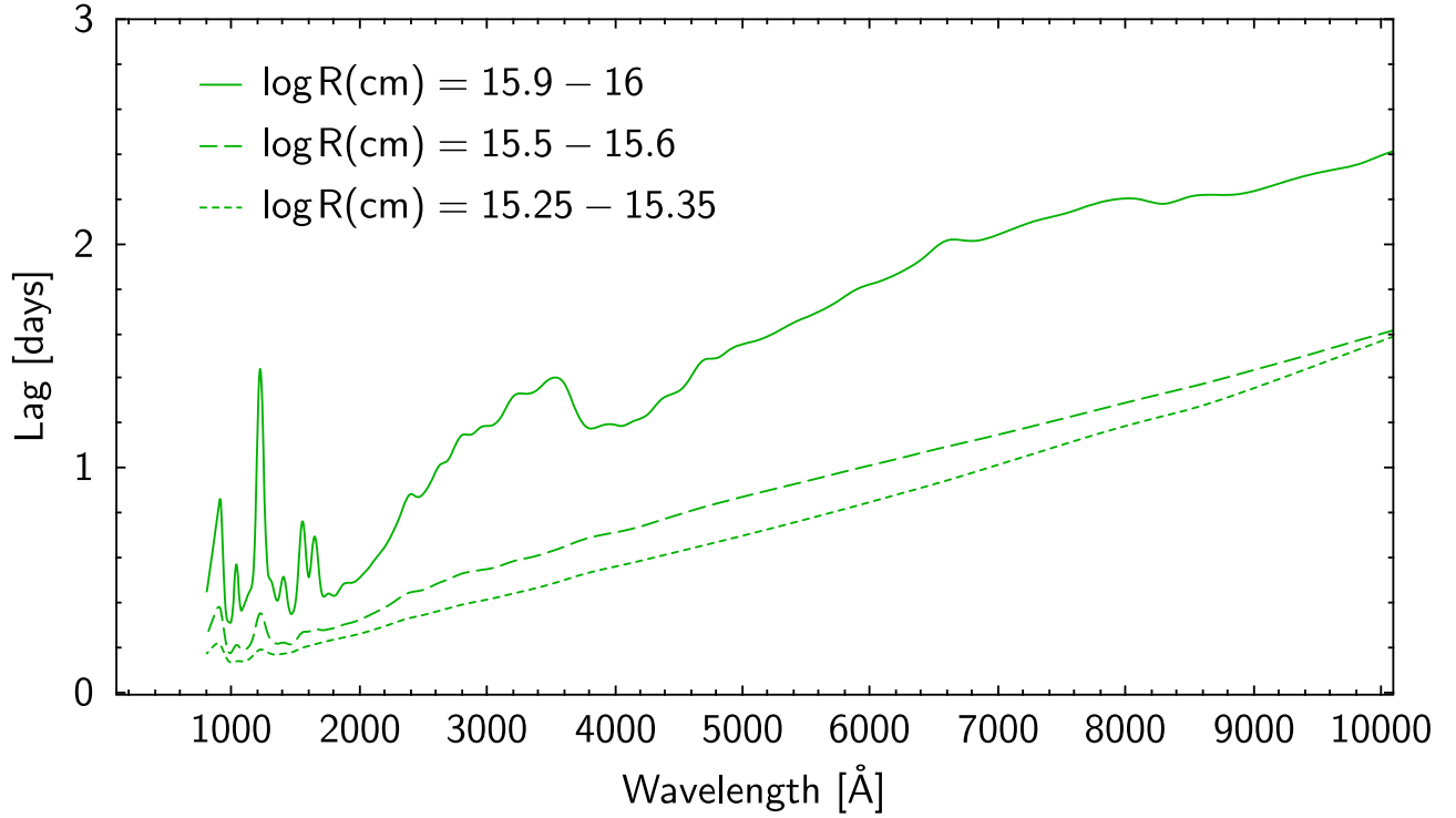
Figure 17. Wavelength-dependent lags for winds with a column density of 10^{24} \text{ cm}^{-2} and distances as marked.
