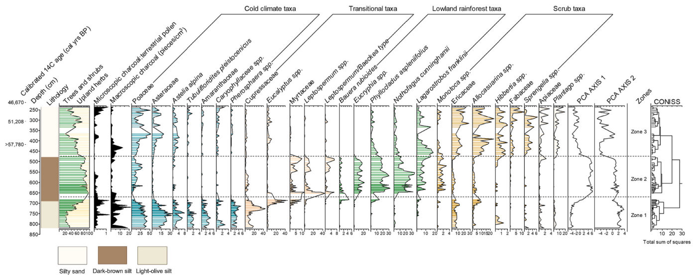
Fig. 4. Darwin Crater pollen and charcoal record including pollen, with >1% abundance. Axis Y represents depth (cm) with corresponding calibrated ^{14}\text{C} ages. Note % scale changes in X axes. The three lithostratigraphic Zones (left) are mirrored by the CONISS defined pollen Zones (right). Total terrestrial pollen is represented by trees and shrubs in green and herbs and upland herbs in yellow. Cold climate taxa are expressed in teal, transitional species in tan, lowland rainforest taxa in green, and scrub taxa in brown. Microscopic and macroscopic charcoal are presented as a ratio of charcoal:terrestrial pollen counts (MC:TP) and pieces/cm ^3 (#/cm ^3 ), respectively. PCA axis 1 (PC1) represents the primary trend within the dataset, responding to shift in temperature and explaining 46% of the variance. PCA axis 2 (PC2) represents the secondary trend within the dataset, responding to change in site type and explaining 18% of variance (see Fig. 6). Note: Gaps in sampling intervals are due to sediment lost in extraction process. For interpretation of the references to colour in this figure legend, the reader is referred to the web version of this article.
