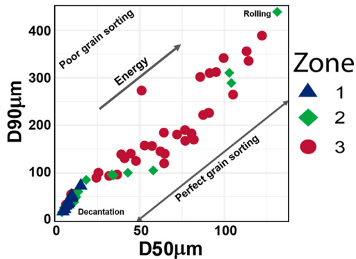
Fig. 2. Grainsize biplot presenting the relationship between coarser (D90 μm) and finer (D50 μm) grain size and hydrodynamic energy (Passeea, 1964), in the sediment Zones of Darwin Crater. For interpretation of the references to colour in this figure legend, the reader is referred to the web version of this article.
