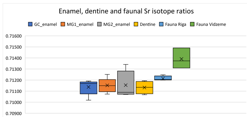
FIGURE 4 Enamel, dentine and faunal ^{87}\text{Sr}/^{86}\text{Sr} ratios, plotted without individual GC_41 Notes: Boxes are formed by the first and the third quartiles; the dividing line shows the median ratio; the whiskers on each box show minimum and maximum ratios; x-mean ratio; N (GC) = 6, N (MG1) = 6, N (MG2) = 6; N (dentine) = 5; N (Fauna Riga) = 4; N (Fauna Vidzeme) = 3 [Color figure can be viewed at wileyonlinelibrary.com ]
