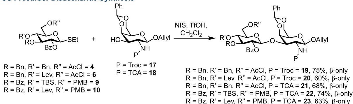
Scheme 3. CS precursor disaccharide synthesis using variously protected CS donors and acceptors and NIS/TfOH glycosylation conditions. Following column chromatography of the crude reactions only \beta -anomer was isolated for compounds 19–22 .
