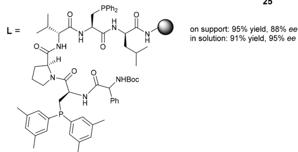
Scheme 4 Palladium-catalysed allylic alkylation of dimethylmalonate with cyclic substrate 3-acetoxycyclopentene using the phosphine-containing \beta -turn peptide Boc-D-Phg-Xps-Pro-D-Val-Pps-D-Leu-OMe – Gilbertson and co-workers. 14
