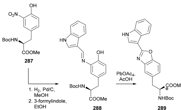
Scheme 57 Synthesis of a benzoxazol-5-yl alanine derivative – Guzov and co-workers. 190
