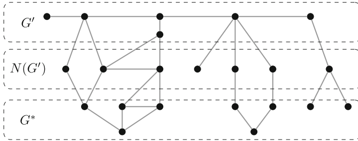
Fig. 13 The decomposition of a graph G into the graphs G' , which is isomorphic to H , the neighbourhood graph N(G') of G' , which is induced by all vertices not in G' but that have one or more neighbours in G' , and the graph G^* induced by the remaining vertices of G
