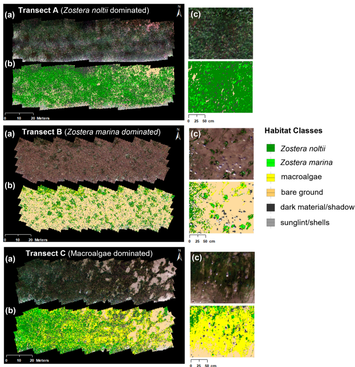
FIGURE 5 (a) Raw multispectral UAV orthomosaic are displayed using the red, green and blue colour composite; (b) classified map using Maximum Likelihood Classifier (MLC); and (c) a close-up example for each transect survey. Transect A, Zostera noltii dominated; Transect B, Zostera marina dominated; Transect C, Macroalgae dominated.
