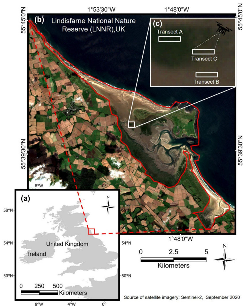
FIGURE 1 (a) Map of the UK showing the location of Lindisfarne National Nature Reserve (LNNR) (red square), (b) LNNR (red boundary outline) indicating the field survey area (white square) and (c) the flight transects surveyed in this study. Transect A, Zostera noltii dominated; Transect B, Zostera marina dominated; Transect C, Macroalgae dominated.
