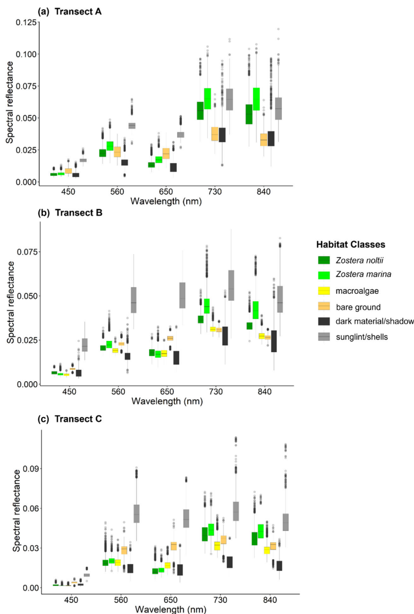
FIGURE 4 Spectral signatures of generated training data including all benthic classes across the multispectral bands for (a) Transect A ( Zostera noltii dominated), (b) Transect B ( Zostera marina dominated) and (c) Transect C (Macroalgae dominated). Boxplots show the median value (horizontal line), the interquartile range representing the dispersion of the data (size of the box), the upper and lower quartiles and outliers.
