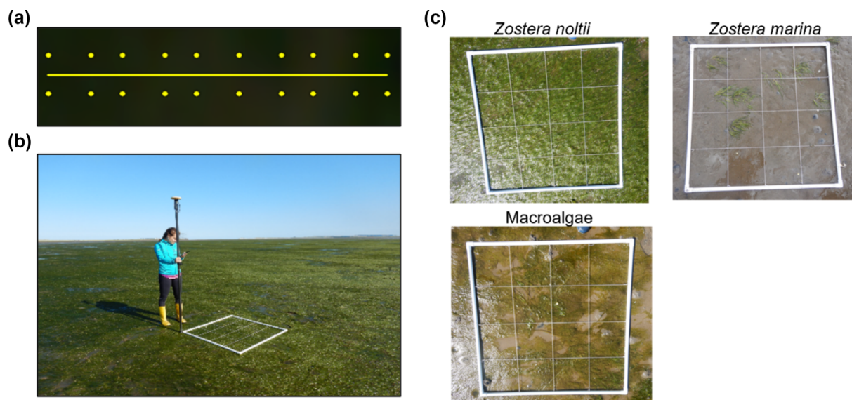
FIGURE 2 (a) Flight transect showing the predefined regular points for photoquadrats ( n = 20 ) across a flight transect. (b) Image showing the quadrat and a Trimble receiver to record the northern corner of the quadrat sample. (c) Photographs of a Zostera noltii , Zostera marina and Macroalgae dominated quadrats.
