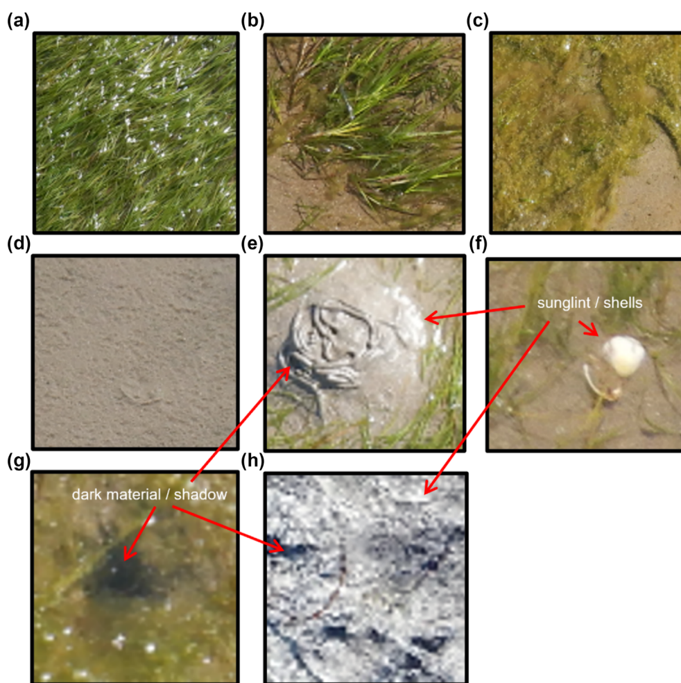
FIGURE 3 Images of benthic substrates initially identified in quadrat photographs before aggregation of benthic classes in further analysis. (a) Zostera noltii , (b) Zostera marina , (c) macroalgae, (d) bare ground, (e) lugworm casts, (f) shells, (g) anoxic sediment and (h) decomposing vegetation. Arrows highlight examples of categories including dark material/shadow and sunglint/shells.
