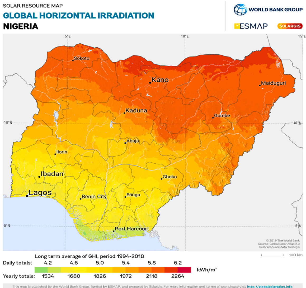
Fig. 3. Average Daily and Annual GHI in Nigeria (Global Solar Atlas, 2024).
