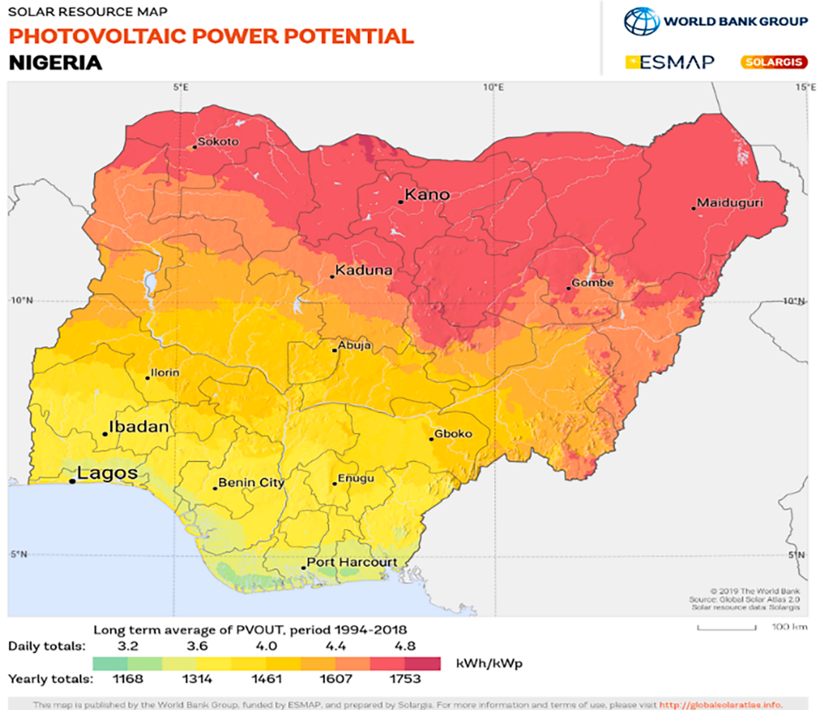
Fig. 5. Average Daily and Annual PVOUT in Nigeria (Global Solar Atlas, 2024).
