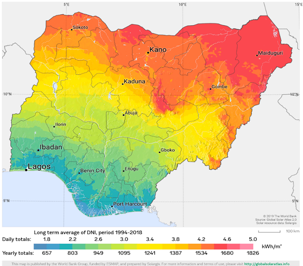
Fig. 4. Average Daily and Annual DNI in Nigeria (Global Solar Atlas, 2024).
