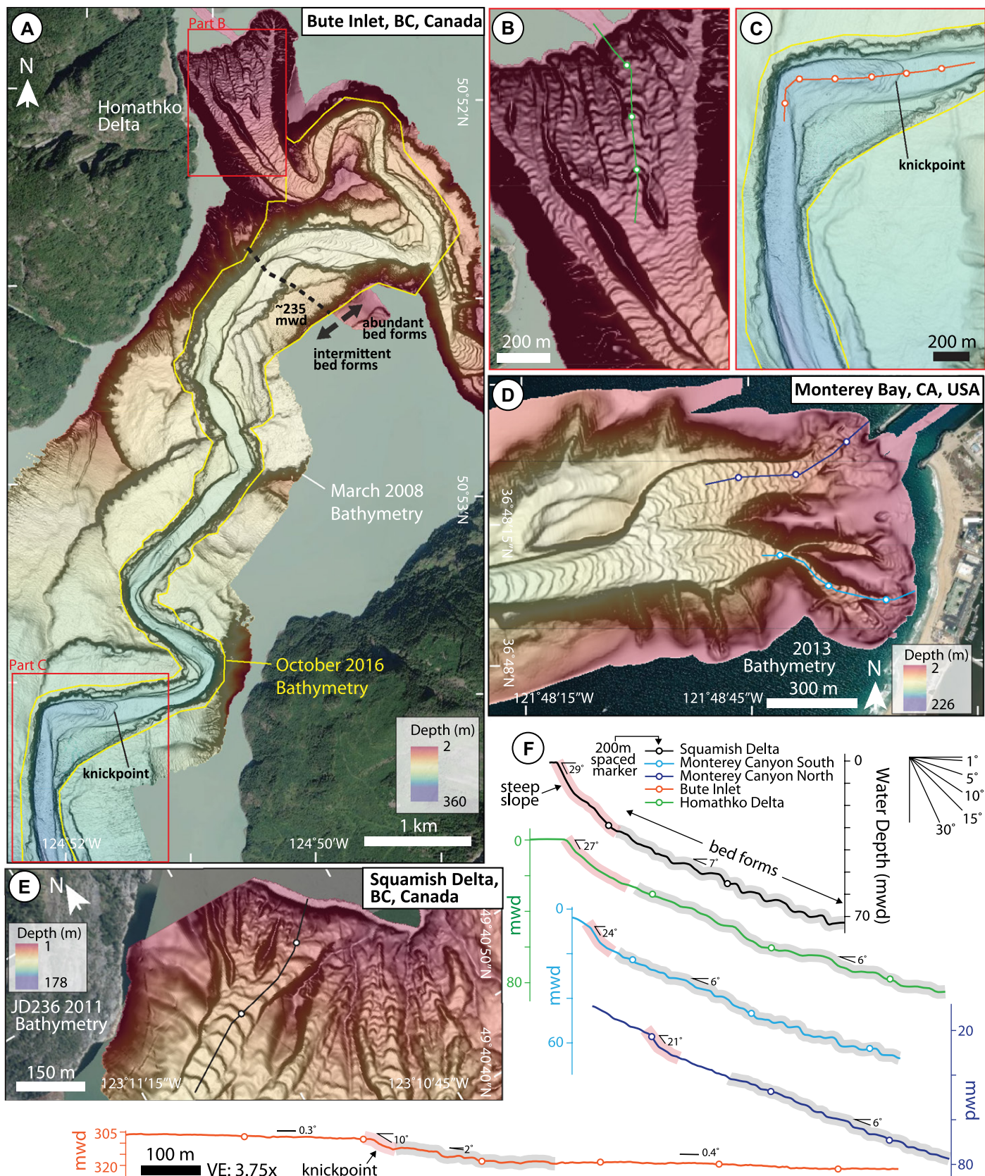
Figure 1. Decameter-scale upstream-migrating bed forms in submarine channels. (A–E) Bathymetric maps showing bed-form distribution in: (A–C) Bute Inlet, British Columbia (BC), where bed forms occur on Homathko Delta (B), proximal channel, and just downstream of knickpoints (C), (D) proximal Monterey Canyon, where bed forms are abundant and start in steep gullies close to shelf edge, and (E) Squamish Delta, where bed forms extend up to steep, smooth Gilbert-type delta. (F) Bathymetric profiles for each example. Positions of profiles are shown in parts A–E. Circles are 200 m spaced horizontal markers on both graphs and maps. Segments containing bed forms correspond to areas of undulations on profiles and crescentic trains on maps. VE—vertical exaggeration; mwd—water depth in meters.
