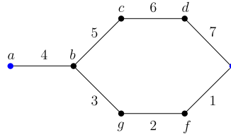
Fig. 8. An example of an optimal labeling of an MSL instance, where the temporal (sub)-graph connecting terminal vertices R = \{a, e\} is neither a tree nor a tree with a C_4 . Note that this is not a solution to ML, as for example there is no temporal path from c to a or to g . Now, we can remove the labels from the edges bg, gf, fe and add them (in the same order) to the edges bc, cd, de , respectively. This way, we obtain an optimal solution, where the subgraph which has labeled edges is a tree (in this case even a path).
