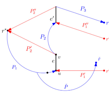
(c) Example of Case A-2-ii.
