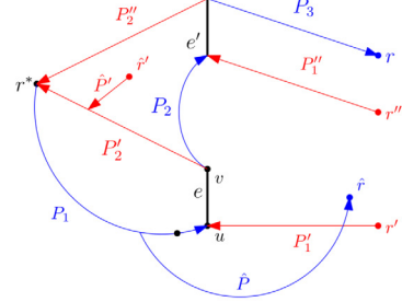
(d) Case A-2-ii(a): P^* from r' to r' either uses no labels from \lambda_{r^*}^+ or no from \lambda_{r^*}^- .
