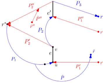
(e) Case A-2-ii(b): P^* from r'' to r' either uses no labels from \lambda_{r^*}^+ or no from \lambda_{r^*}^- .
