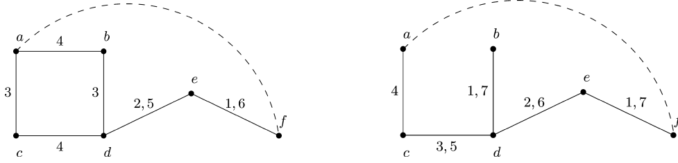
(a) An example of a labeling that temporally connects a graph that contains a C_4 , where the C_4 edges receive one label and all other edges of a spanning tree receive two labels. (b) An example of a labeling that temporally connects a graph that does not contain a C_4 , where one edge receives one label and all other edges of a spanning tree receive two labels.
