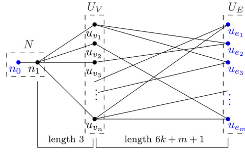
Fig. 7. Illustration of the MSL instance produced by the reduction presented in the proof of Theorem 14, where the blue vertices represent set R^* . (For interpretation of the colors in the figure(s), the reader is referred to the web version of this article.)
