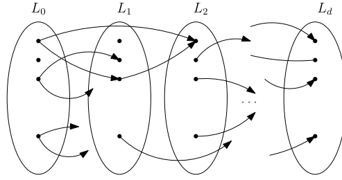
Fig. 2. Example of a canonical layering.
