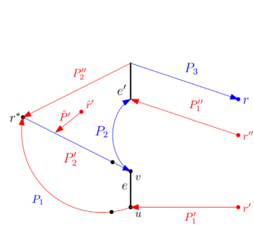
(b) Modification of Case A-2-iii.
