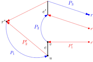
(a) Example of Case A-2-i.
