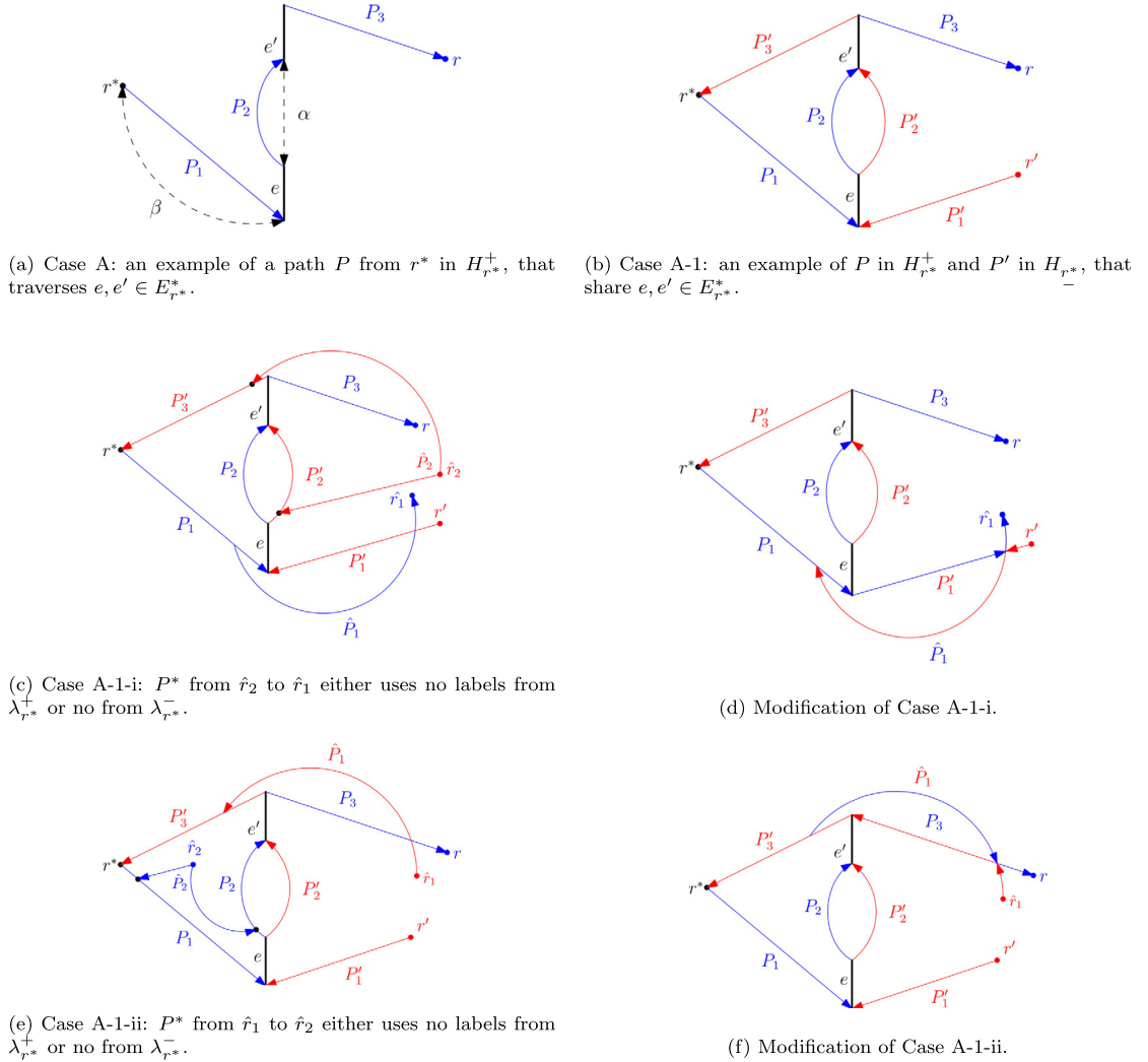
Fig. 9. Cases A-1 – A-1-ii, where blue color corresponds to the labeling \lambda_{r^*}^+ and red to \lambda_{r^*}^- .
