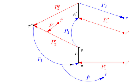
(a) Case A-2-iii: P^* from r' to r either uses no labels from \lambda_{r^*}^+ or no from \lambda_{r^*}^- .
