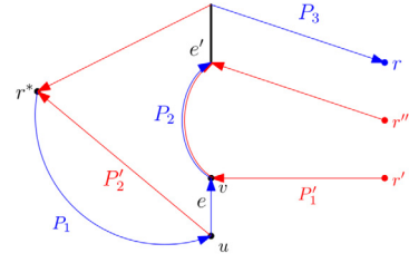
(b) Modification of Case A-2-i.
