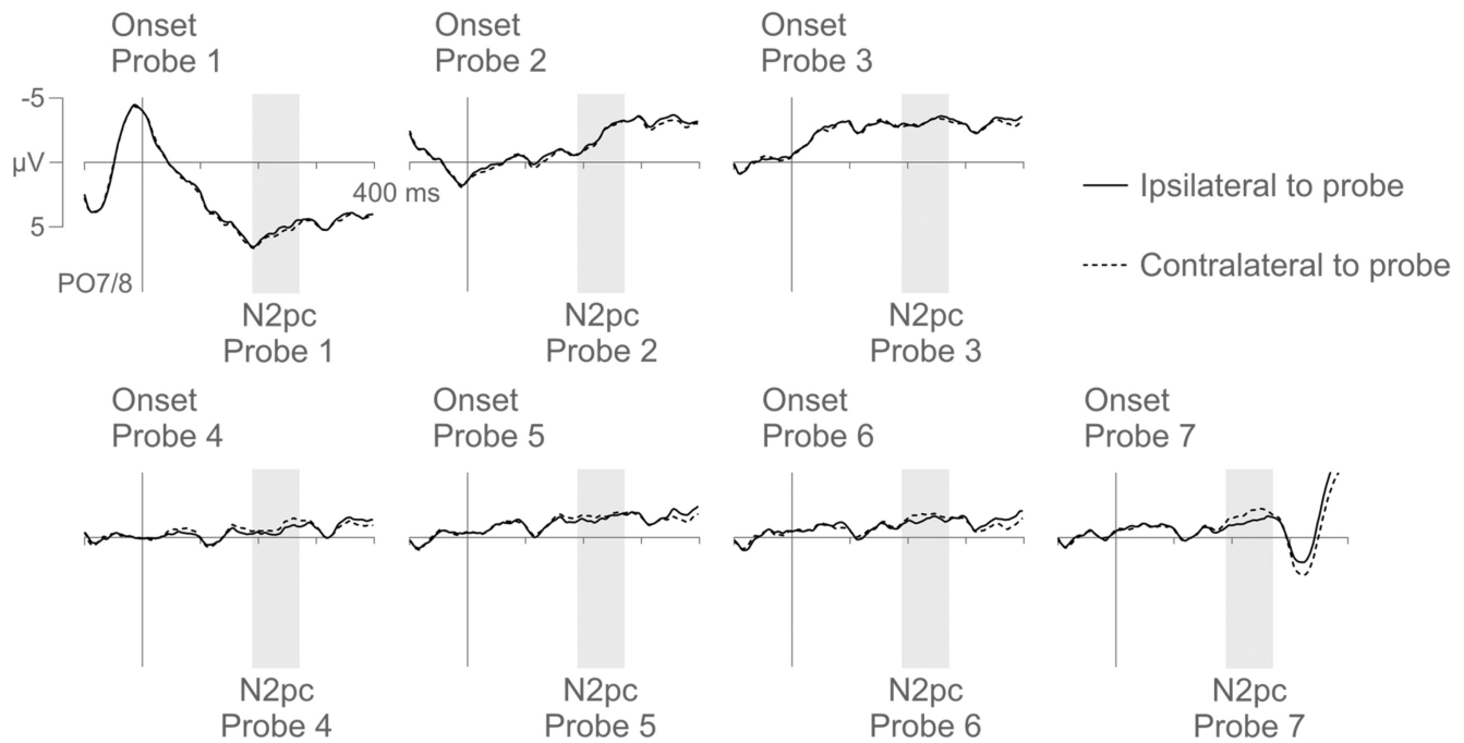
FIGURE 3 Grand-averaged ERPs elicited by relevant target color probes in color repetition trials of Experiment 1 at electrodes PO7/8 contralateral and ipsilateral to color singleton probes in each of the seven probe displays presented between consecutive search displays. Probe 1 is the first probe to follow the previous search display and probe 7 is the probe to immediately precede the next search display. Shaded areas mark N2pc time windows (190–270 ms after onset of each individual probe).
